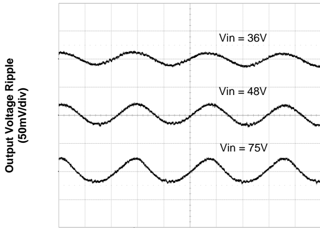
Figure 3. Output Ripple Voltage at Full Load
