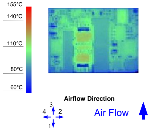
Figure 8. Thermal Image for Airflow Direction 3 (22A output, 55°C ambient, 0 LFM, typical Vin, open frame, unit soldered onto a fixture board)
