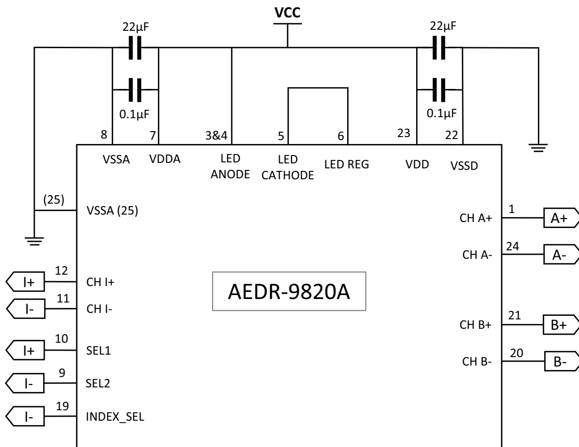
Figure 5: Reference Schematic Diagram for AEDR-9820A
