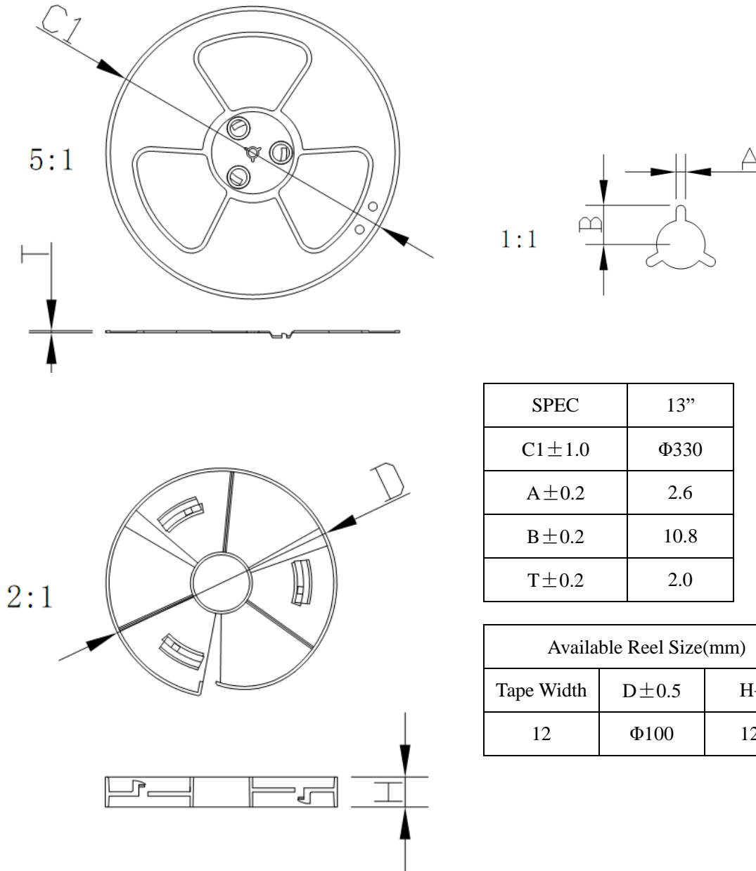
Figure 5. Tape Specification
