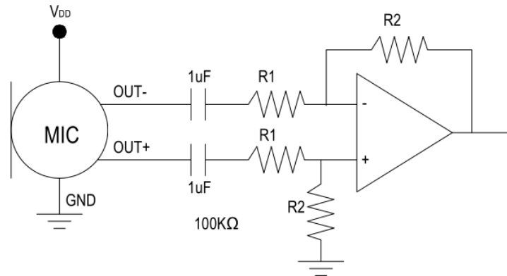
Figure 4. Recommended interface circuit for customers' applications
