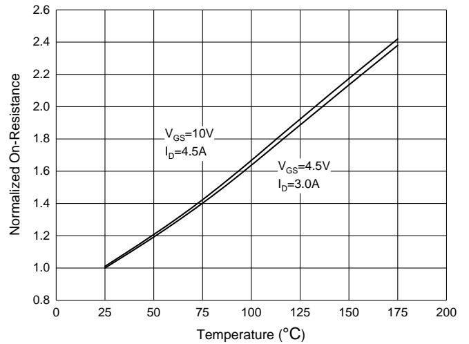
Fig. 6 - R_{DS(ON)} - Temperature
