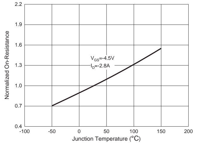
Fig. 4 - R_{DS(ON)} —Temperature
