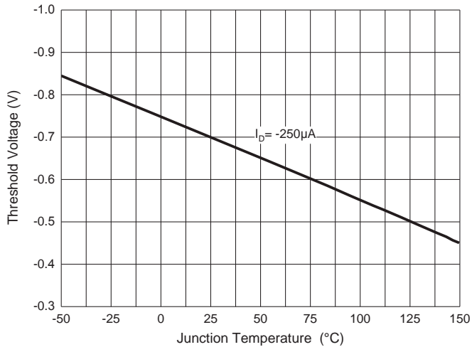
Fig. 5 - Threshold Voltage
