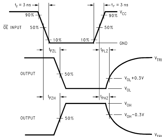
Figure 6. AC Waveforms
