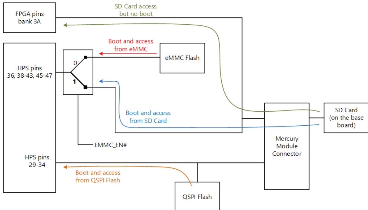
Figure 10: Boot Modes
