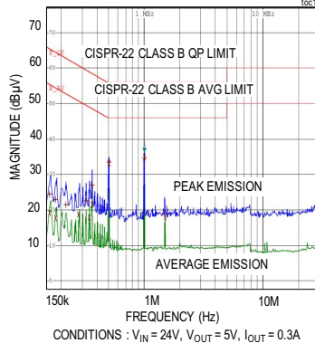
CONDUCTED EMISSION PLOT (EMI FILTER C = 0.1\mu F + 0.68\mu F , L = 82\mu H , C = 1\mu F )
