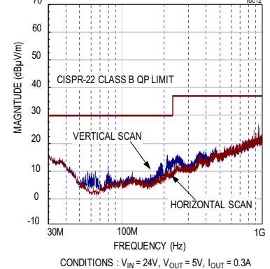
RADIATED EMISSION PLOT ( C6 = 0.1\mu F , C7, C8, C9 = OPEN , L1 = SHORT )
