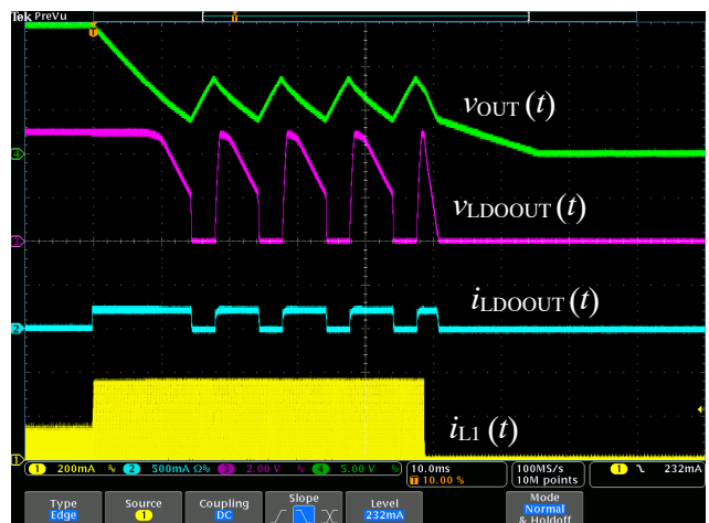
Figure 34. LDO Over-current Protection – Over-loaded LDO Rail, I_{OUT} = 30\text{mA} , I_{LDOOUT} = 30\text{mA} , V_{IN} = 230\text{V}
