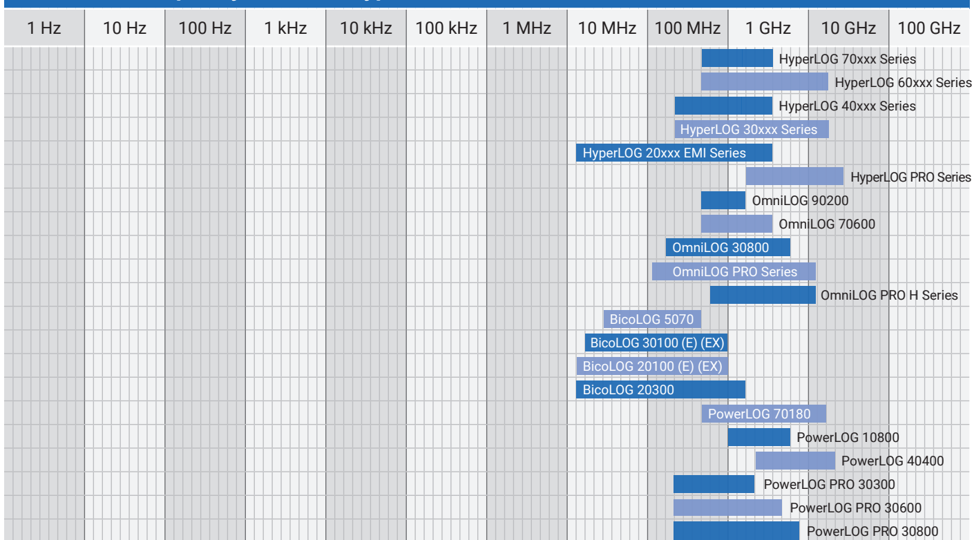
Frequency Overview HyperLOG®, BicoLOG® and PowerLOG® Antennas
