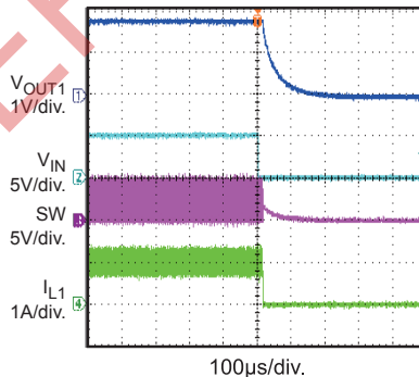
Enable down I_{OUT1} = 1A , I_{OUT2} = 0A
