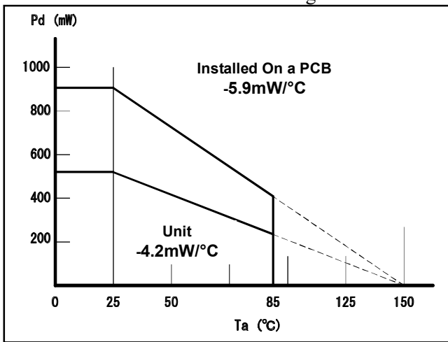
Figure 6. SOT23-5
