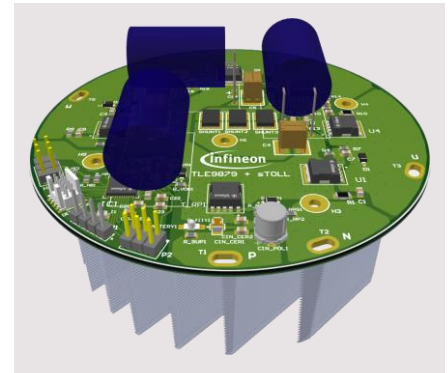
Figure: Reference design for engine cooling fan
