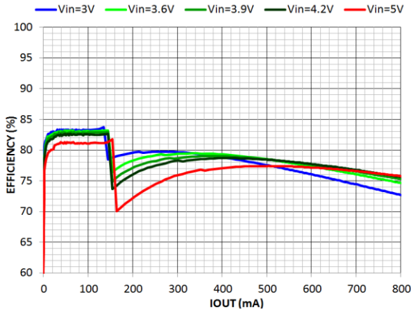
Figure 21. Efficiency vs. Output Current V_{OUT} = 0.8\text{ V} , \text{Temp} = 25^\circ\text{C}
