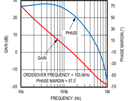
LV BUCK BODE PLOT ( V_{IN} = 5V , V_{OUT} = 1.8V , MODE = PWM, LOAD = 1A)
