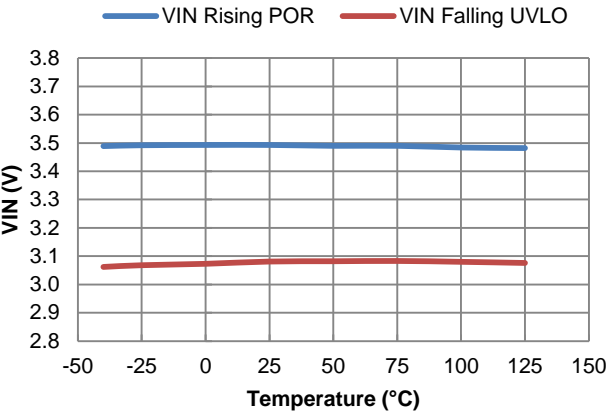
Figure 7. VIN Power-On Reset and UVLO vs. Temperature
