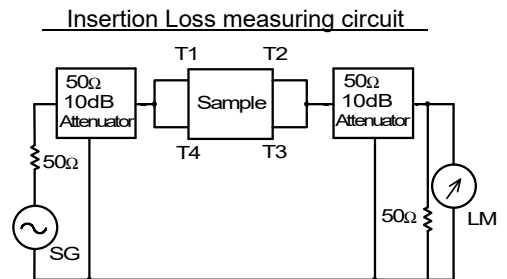
Measuring circuit (based on MIL-STD-220)
