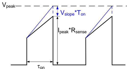
Typical Waveform
