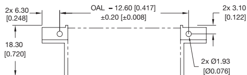
MALE INSULATOR FOR PCB MOUNT CONNECTOR
