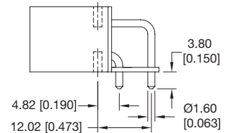
SIZE 16 CONTACTS DUAL ROW
