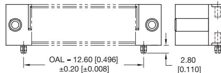
RIGHT ANGLE (90°) PCB MOUNT CONNECTOR
