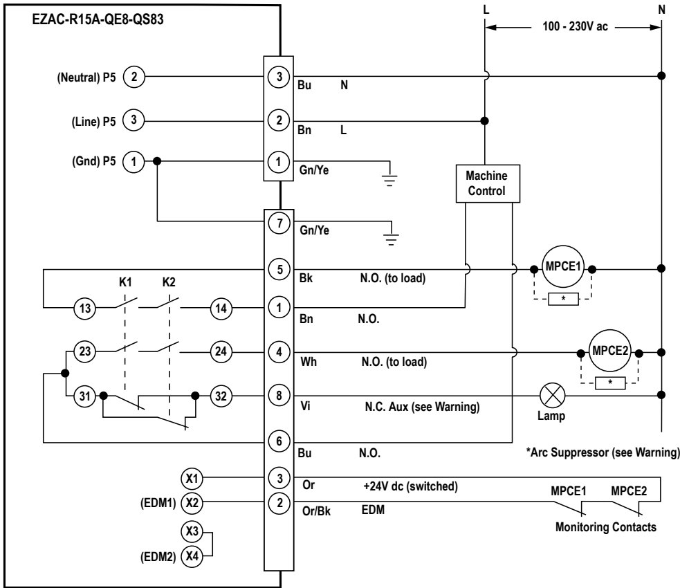
Figure 9. Wiring—model EZAC-R15A-QE8-QS83
