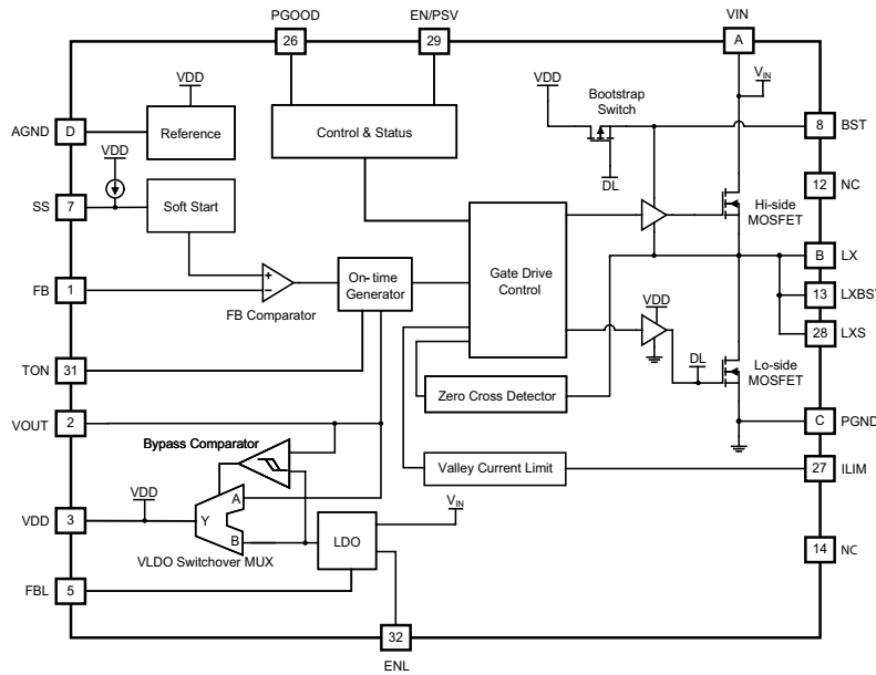
SiC401A/B Functional Block Diagram
