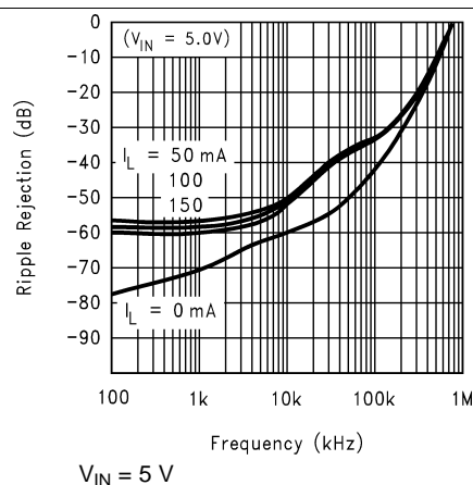
Figure 18. Ripple Rejection
