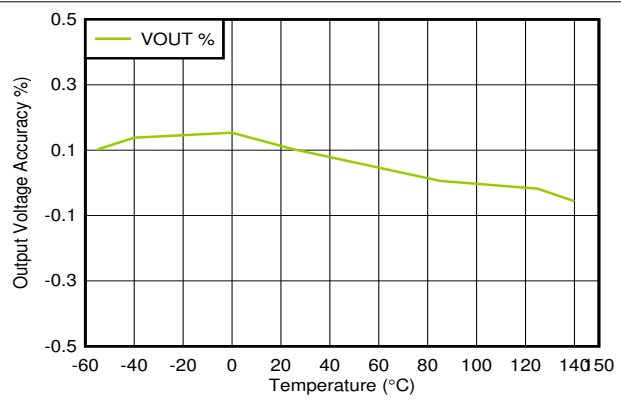
Figure 6-30. Output Accuracy vs Temperature
