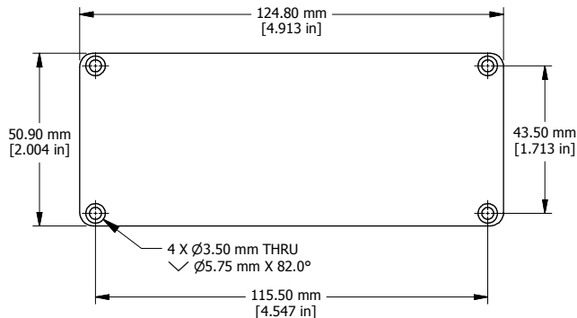
END PLATE
