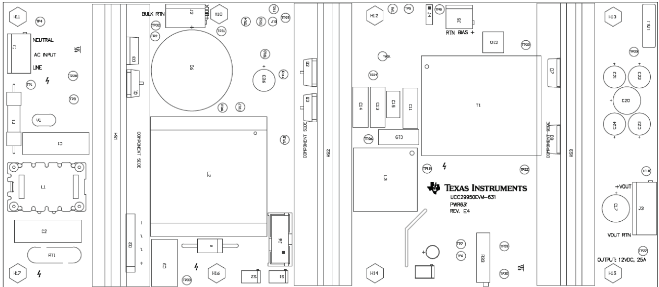
Figure 34. UCC29950EVM-631 Top Layer Assembly Drawing (top view)
