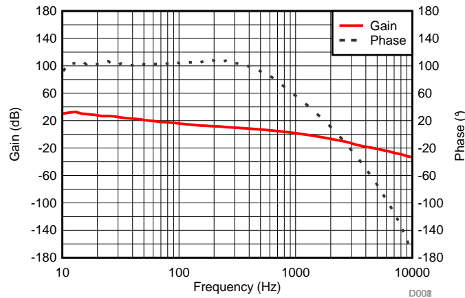
Figure 11. Gain/Phase vs. Frequency
