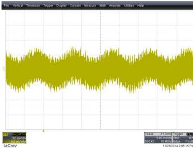
Figure 30. V_{OUT} 25 A, Aux Bias
