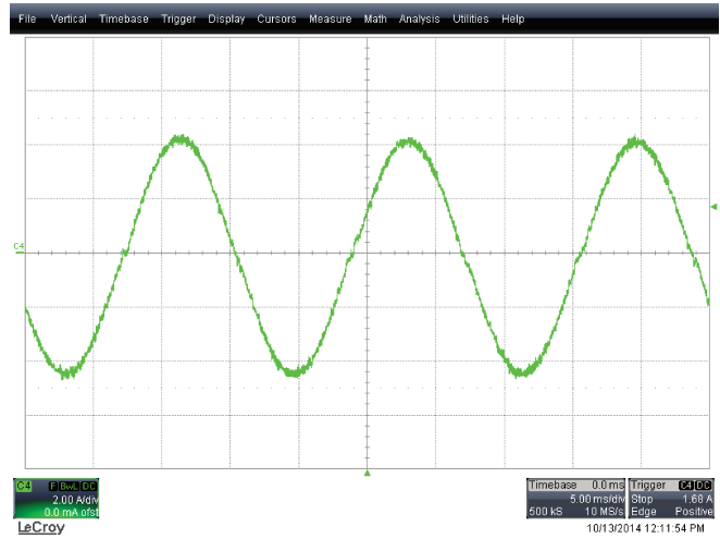
Figure 20. UCC29950EVM-631 Input Current (115-V AC , 60-Hz, full load 2 A/div.)
