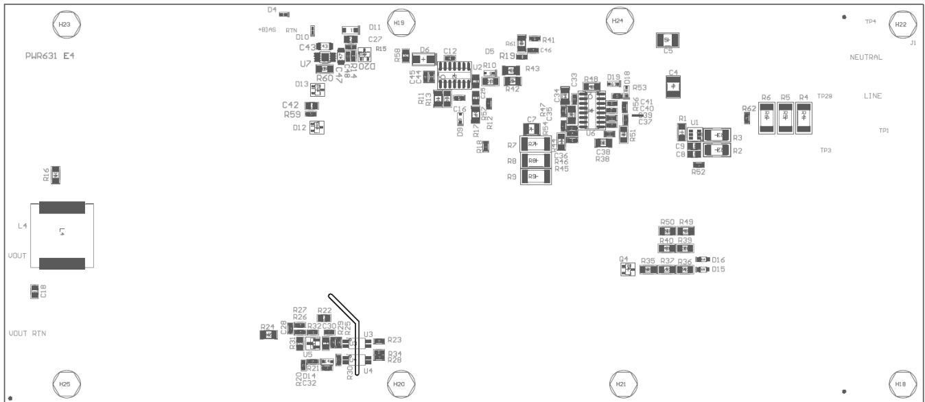
Figure 35. UCC29950EVM-631 Bottom Layer Assembly Drawing (bottom view)
