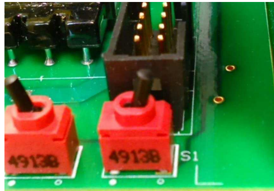
Figure 7. S1 and S2 Settings for PFC and LLC on (Aux Bias Mode and Self Bias Mode)
