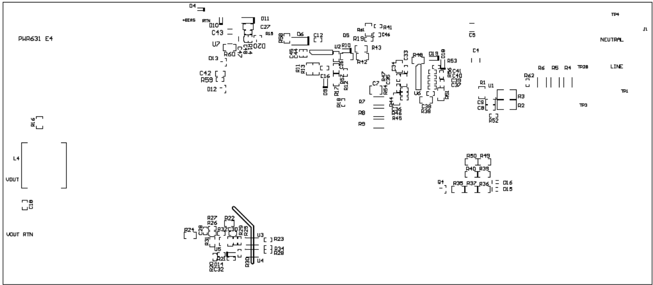
Figure 38. Components Assembly
