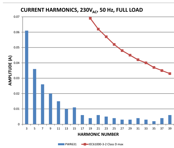
Figure 15. UCC29950EVM-631 Current Harmonics (230-V AC , 50-Hz input, full load)
