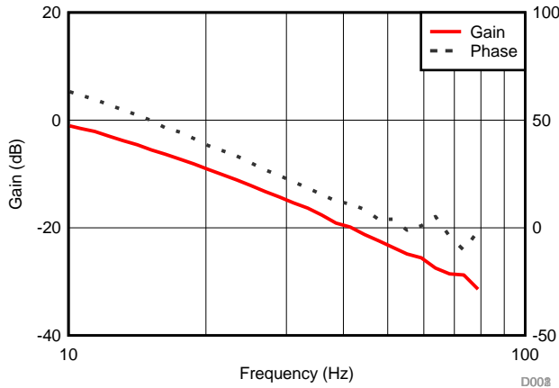
Figure 9. PFC Loop Gain/Phase at 300 W, 115 V
