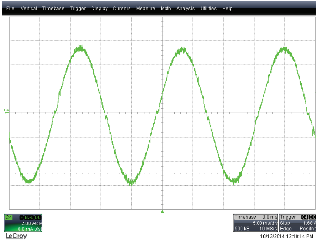
Figure 19. UCC29950EVM-631 Input current (90-V AC , 60-Hz, full load, 2 A/div.)
