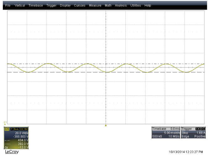
Figure 23. UCC29950EVM-631 V BULK Voltage Ripple (230-V AC , 50-Hz input, full load)
