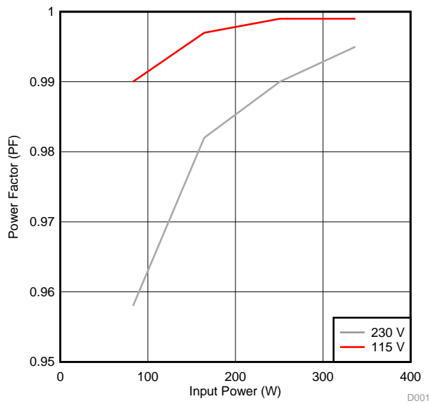
Figure 18. Power Factor vs Input Power
