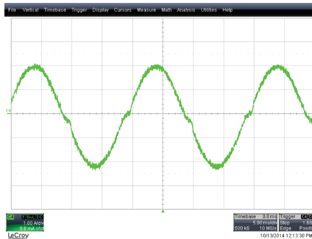
Figure 21. UCC29950EVM-631 Input Current (230-V AC , 50-Hz, full load 1 A/div.)
