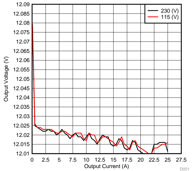
Figure 17. Load Regulation vs Output Current
