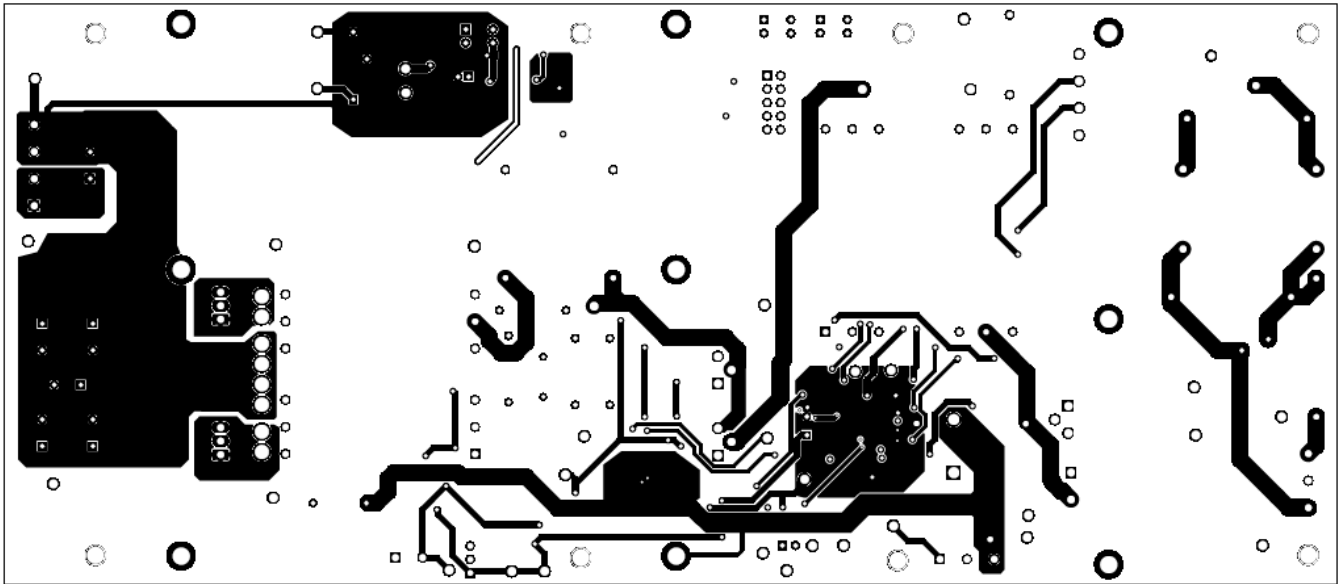
Figure 36. UCC29950EVM-631 Top Copper (top view)
