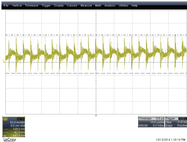
Figure 24. UCC29950EVM-631 Output Noise (115-V AC , 60-Hz input, full load)
