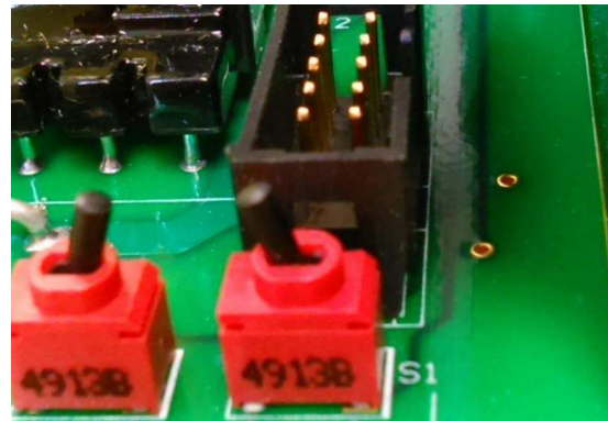
Figure 8. S1 and S2 Settings for PFC Stage On, LLC Stage Off (Aux Bias Mode only)
