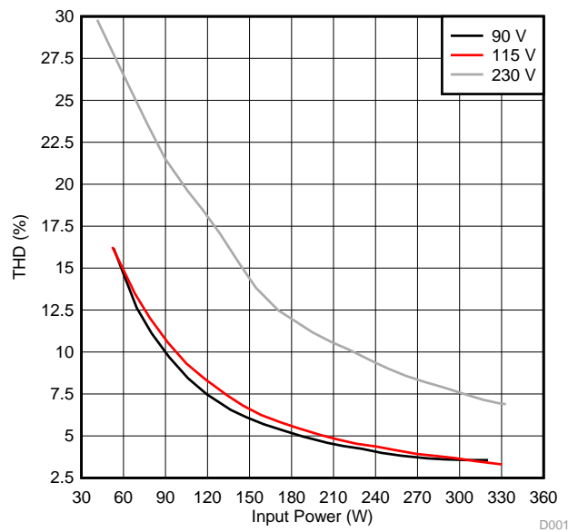
Figure 14. UCC29950EVM-631 Total Harmonic Distortion (as a function of line voltage and load current)
