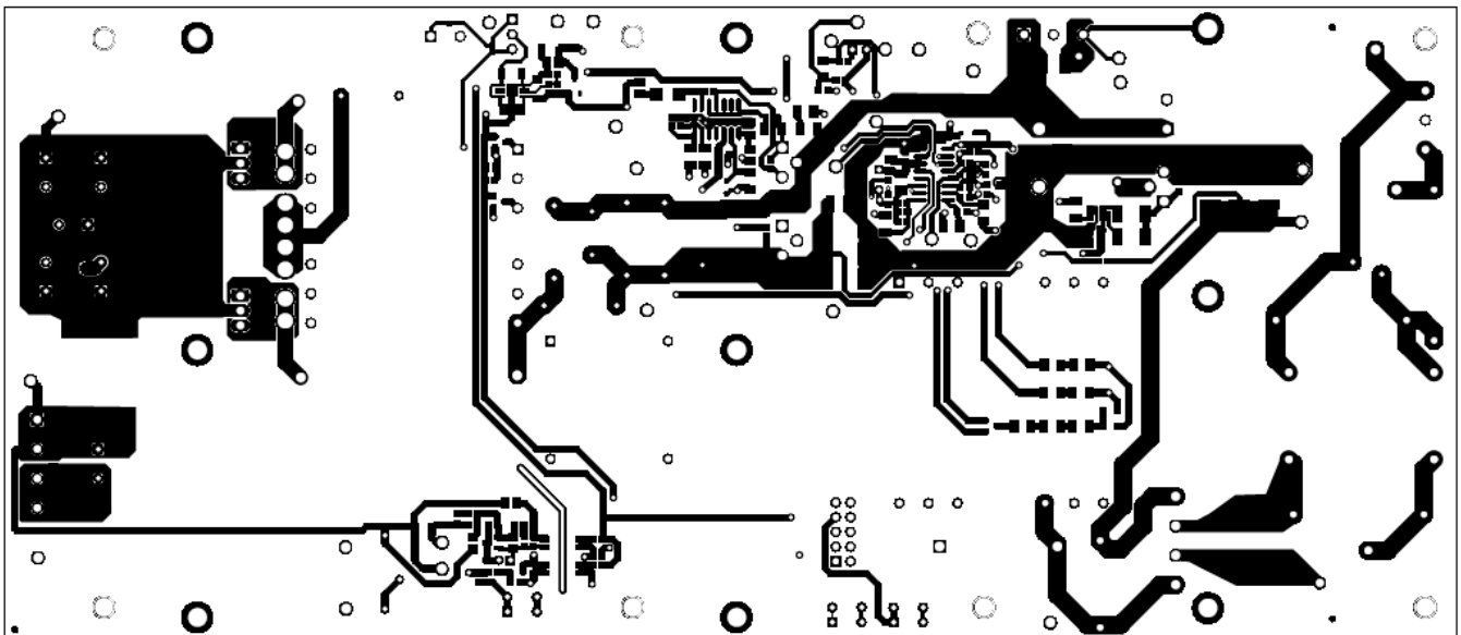
Figure 37. UCC29950EVM-631 Bottom Copper (bottom view)
