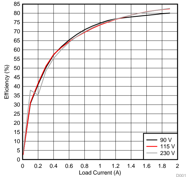
Figure 13. UCC29950EVM-631 Typical Light-Load Efficiency (as a function of line voltage and current)
