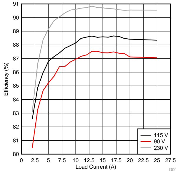
Figure 12. UCC29950EVM-631 Typical Efficiency (as a function of line voltage and current)
