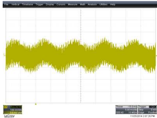
Figure 33. V_{OUT} 25 A, Aux Bias
