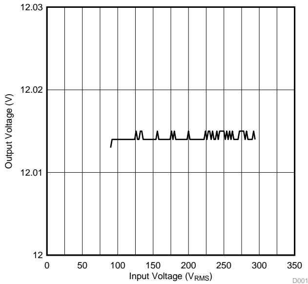
Figure 16. Line Regulation vs Input Voltage
