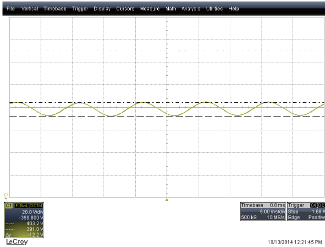
Figure 22. UCC29950EVM-631 V BULK Voltage Ripple (115-V AC , 60-Hz input, full load)
