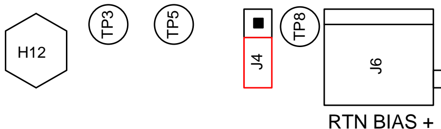
Figure 5. J4 Link Setting for Self Bias Mode
