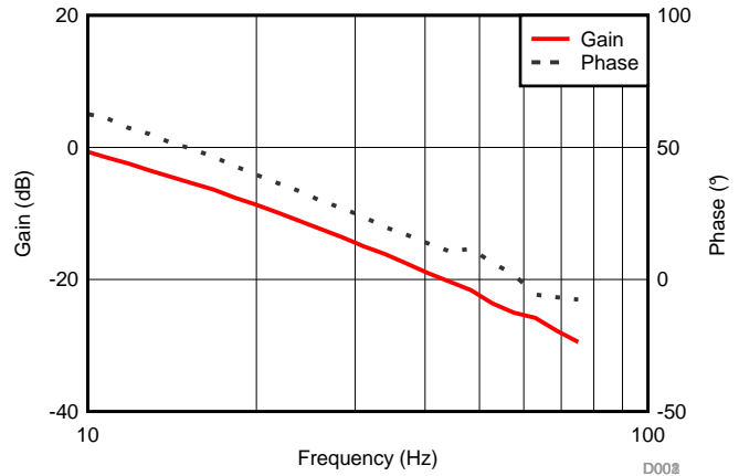
Figure 10. PFC Loop Gain/Phase at 300 W, 230 V
