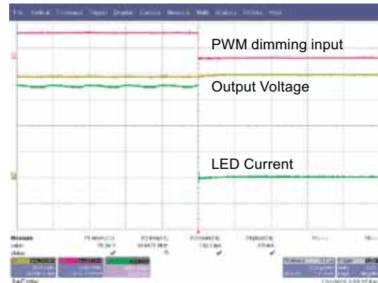
Fig. 8b: Fall time of LED Current at 80V output ( 5\mu\text{s}/\text{div} )
