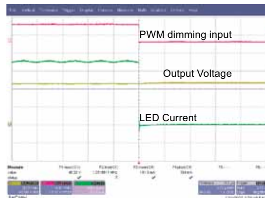
Fig. 9b: Fall time of LED Current at 40V output ( 5\mu\text{s}/\text{div} )
