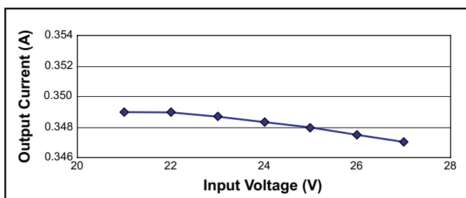
Fig. 4. Output Current vs. Input Voltage
