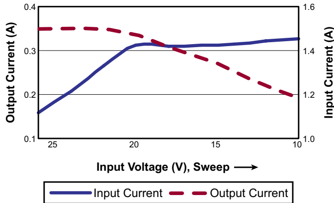
Fig. 5. Input Under Voltage Behavior
