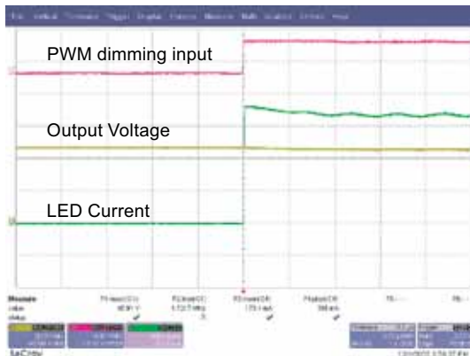
Fig. 9a: Rise time of LED Current at 40V output ( 5\mu\text{s}/\text{div} )
