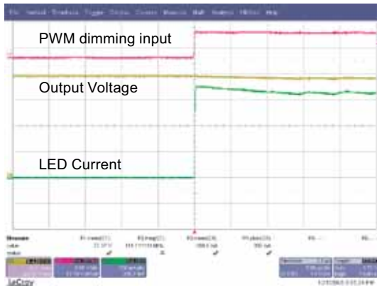
Fig. 8a: Rise time of LED Current at 80V output ( 5\mu\text{s}/\text{div} )
