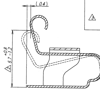
SECT. A-A
