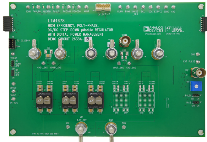
Figure 1. 3x LTM4678; 150A DC2638A-B Demo Circuit
