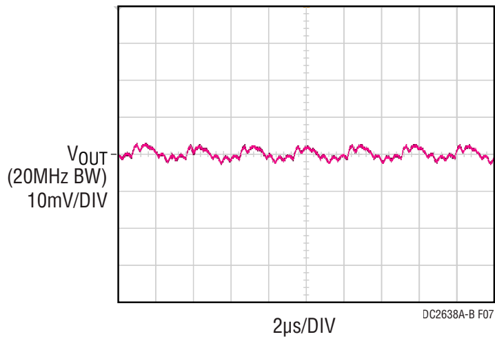
Figure 7. Output Voltage Ripple @ V_{IN} = 12V , V_{OUT} = 1V , I_{OUT} = 150A , f_{SW} = 350kHz
