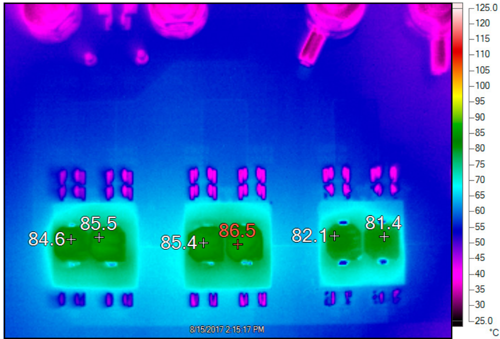
Figure 8. Thermal @ V_{IN} = 12V , V_{OUT} = 1.0V , I_{OUT} = 100A , T_A = 25^{\circ}C , No Airflow
