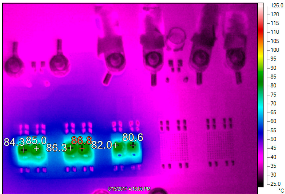
Figure 9. Thermal @ V_{IN} = 12V , V_{OUT} = 1.0V , I_{OUT} = 140A , T_A = 25^{\circ}C , 400LFM Airflow
