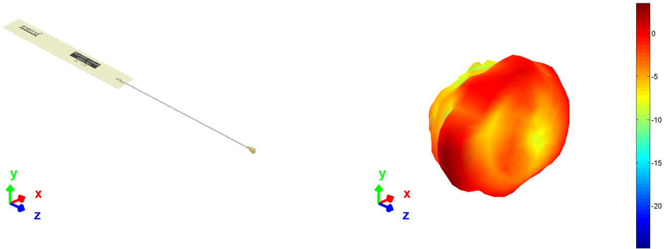
3D pattern at 2340MHz
