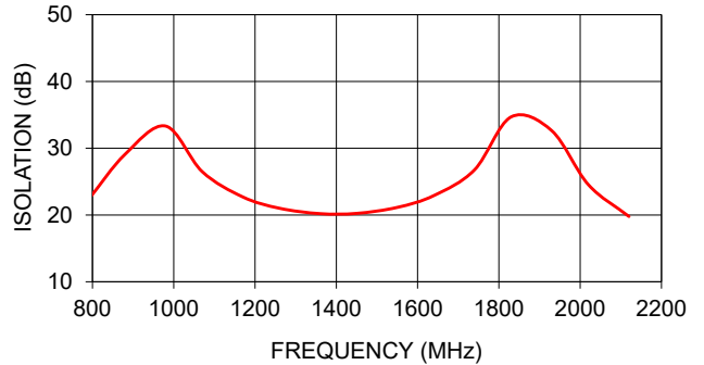
GP2S+ ISOLATION
