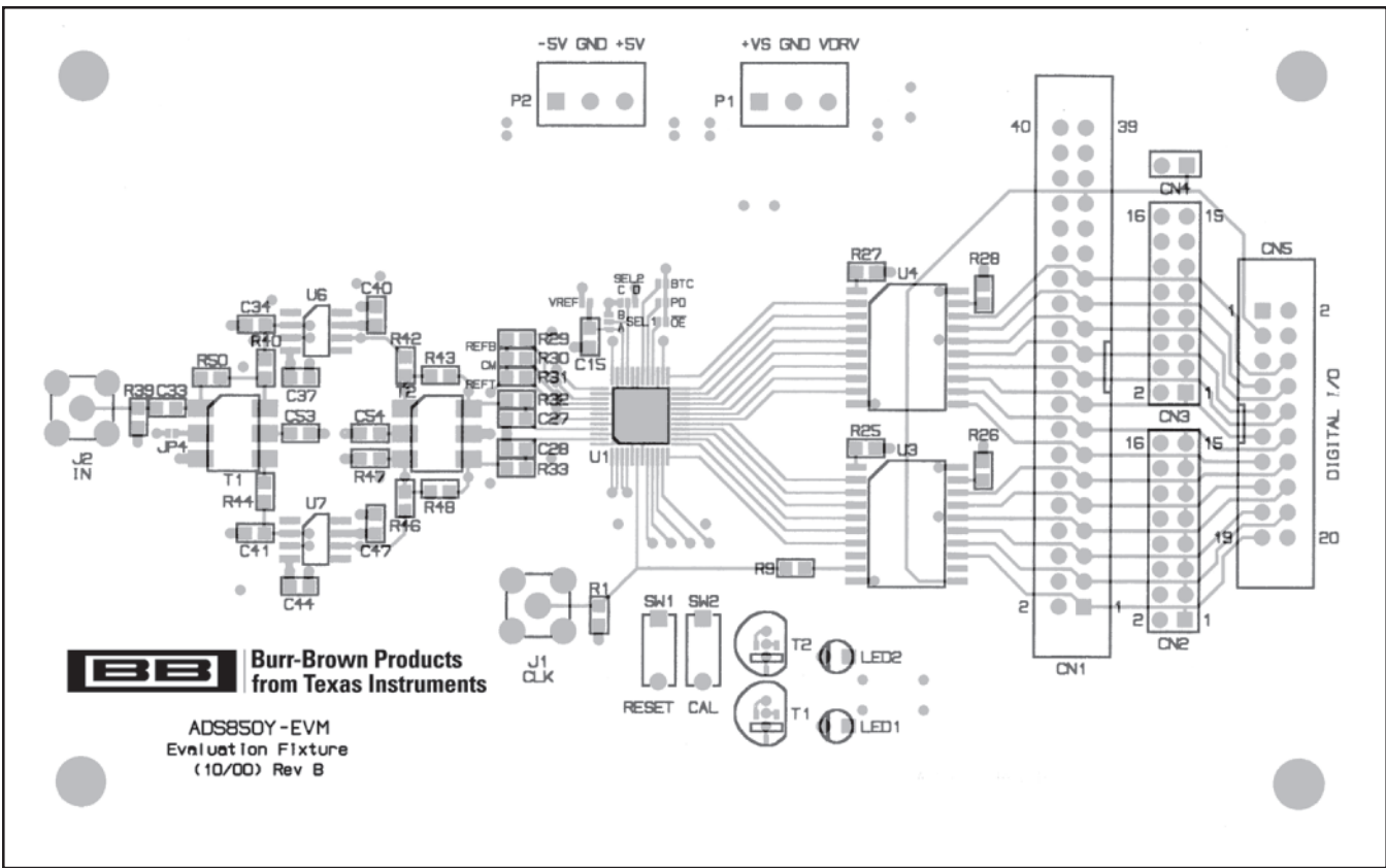
FIGURE 2. Top Layer with Silkscreen.
