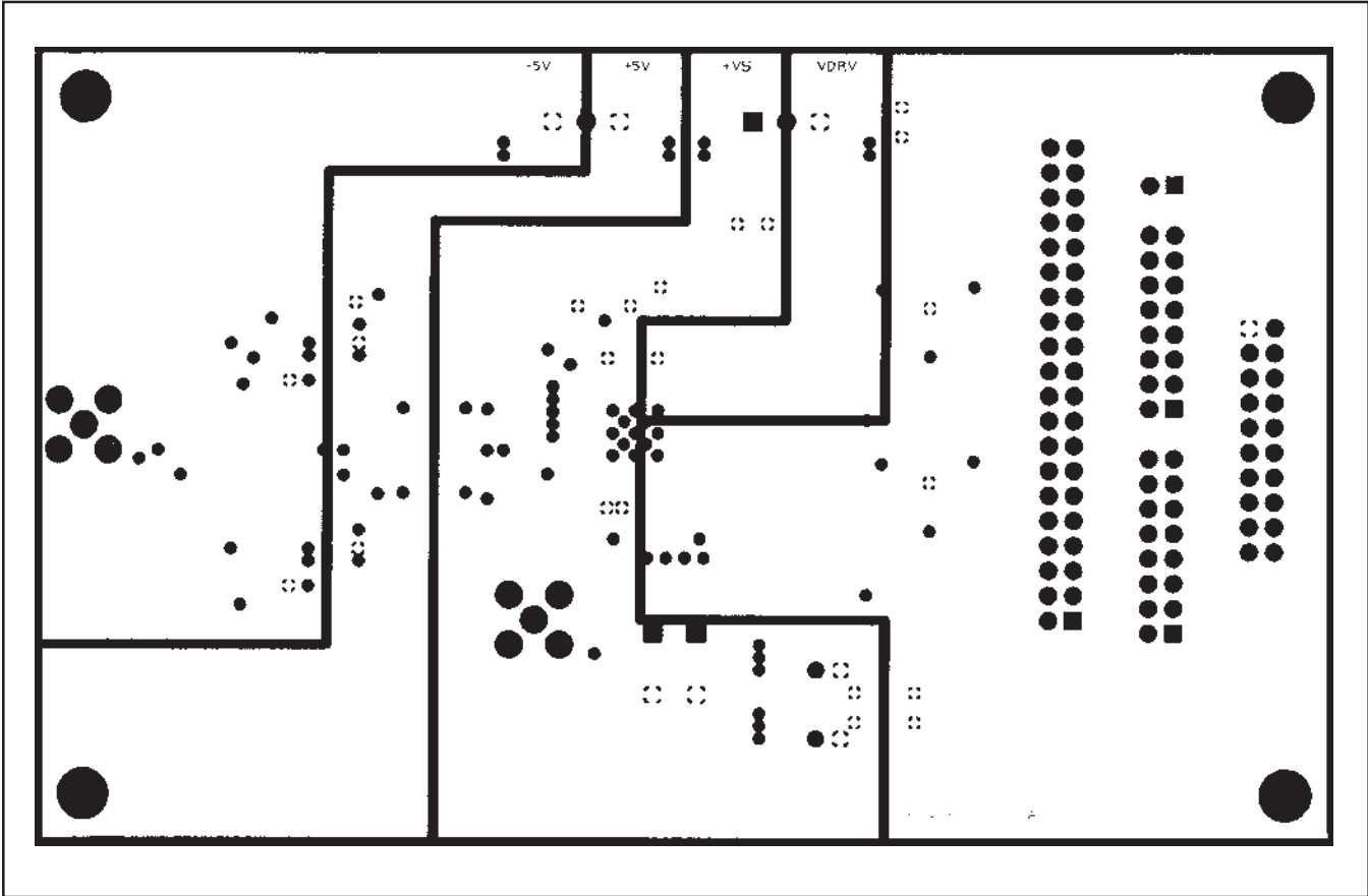
FIGURE 3. Power Plane.
