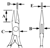
2642S Flat tip "Duck Bill" pliers
