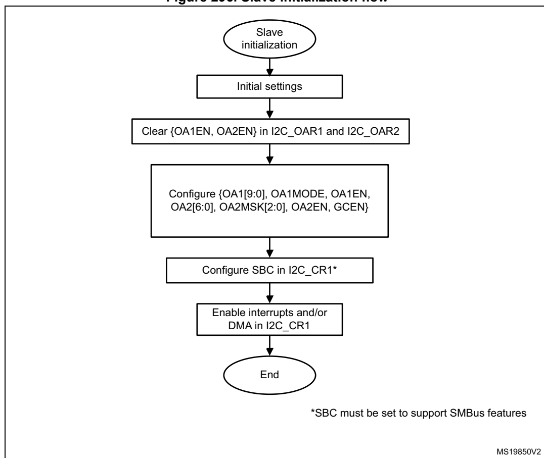
Figure 296. Slave initialization flow
