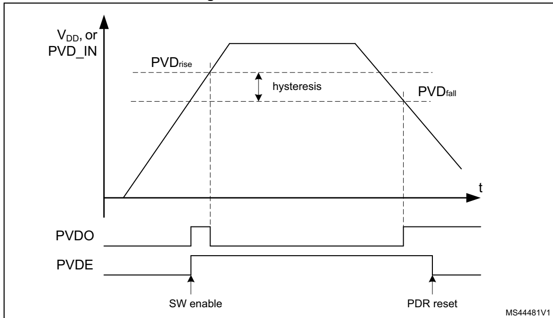
Figure 10. PVD thresholds
