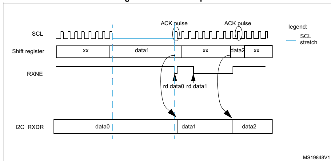
Figure 294. Data reception
