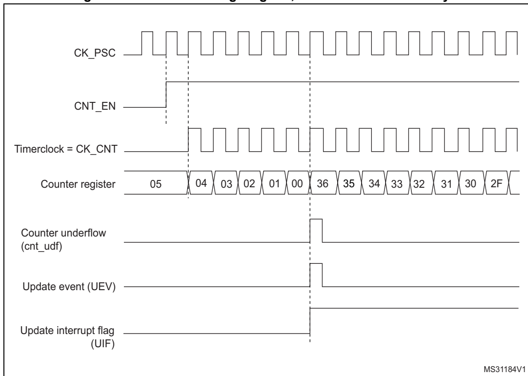
Figure 154. Counter timing diagram, internal clock divided by 2
