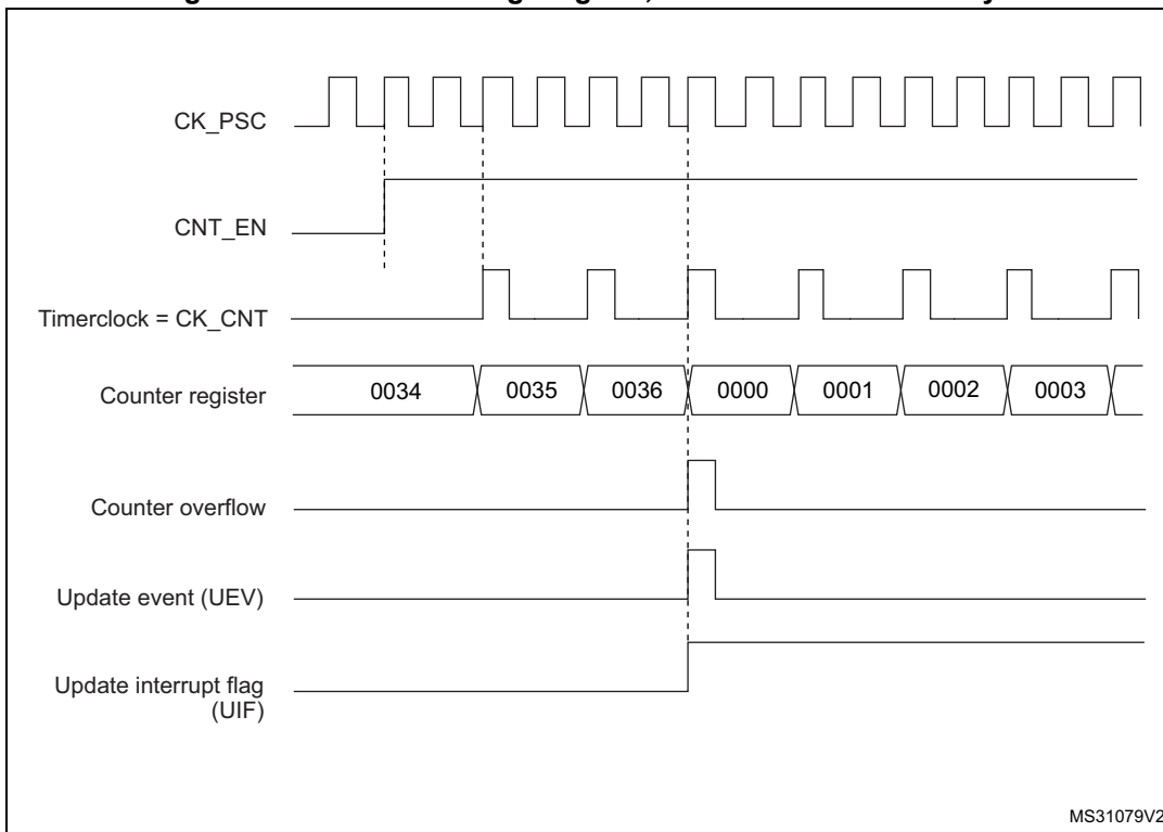
Figure 208. Counter timing diagram, internal clock divided by 2
