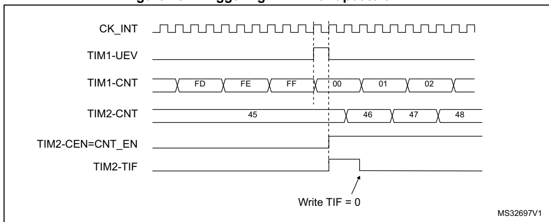
Figure 251. Triggering TIM2 with update of TIM1
