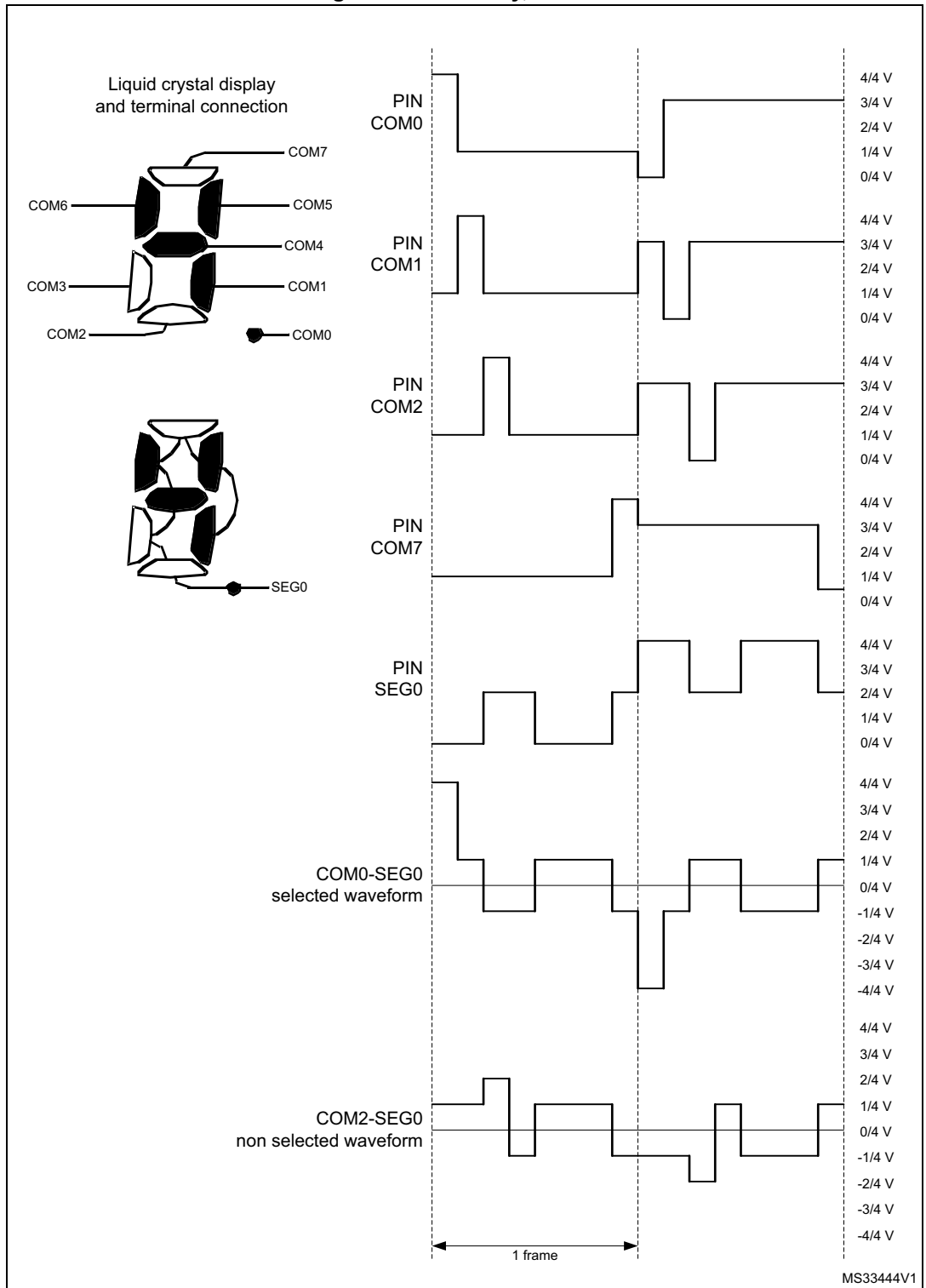
Figure 103. 1/8 duty, 1/4 bias
