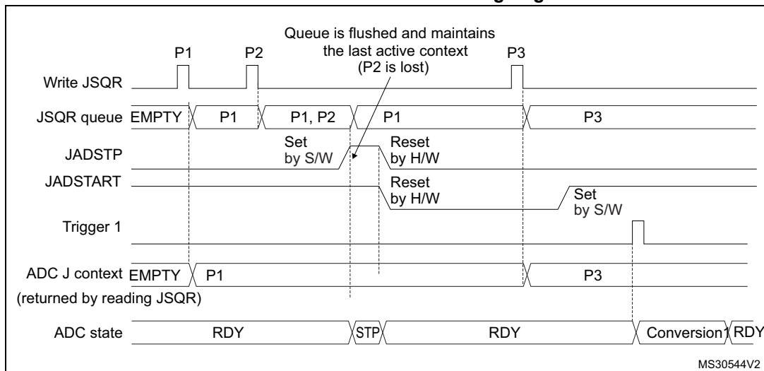
Figure 59. Flushing JSQR queue of context by setting JADSTP = 1 (JQM = 0) Case when JADSTP occurs outside an ongoing conversion
