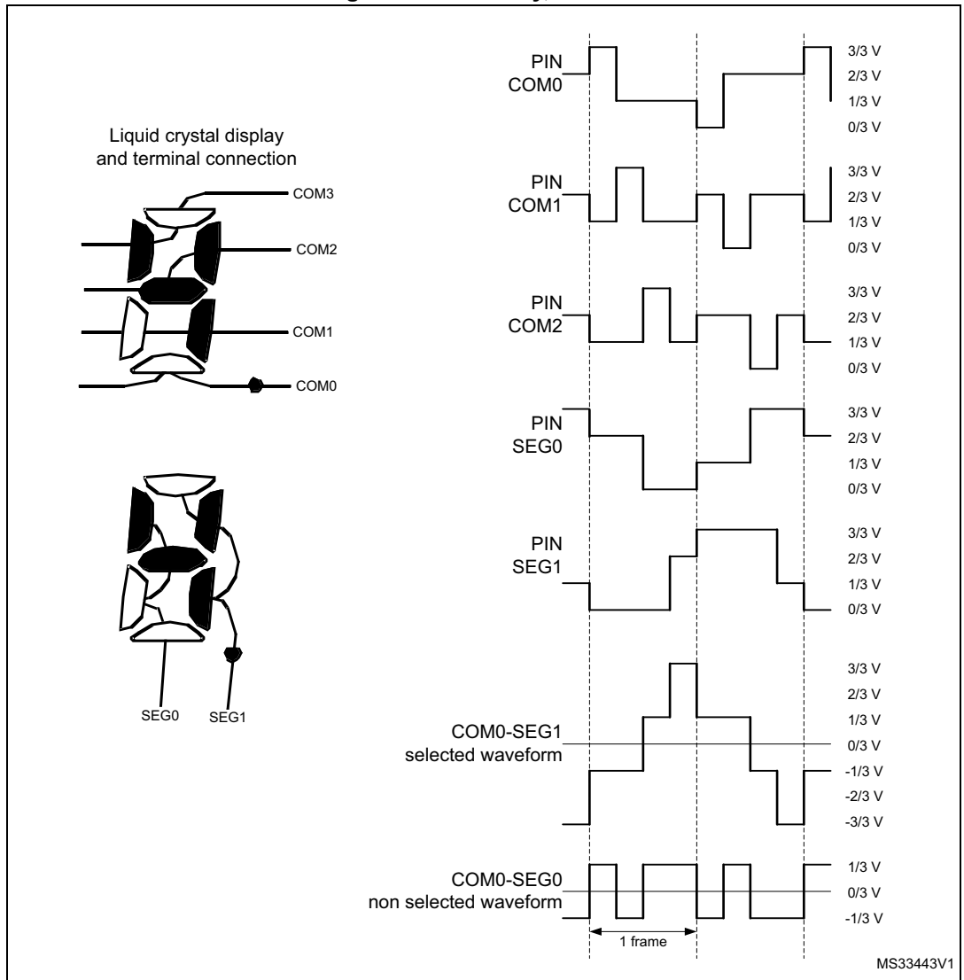
Figure 102. 1/4 duty, 1/3 bias
