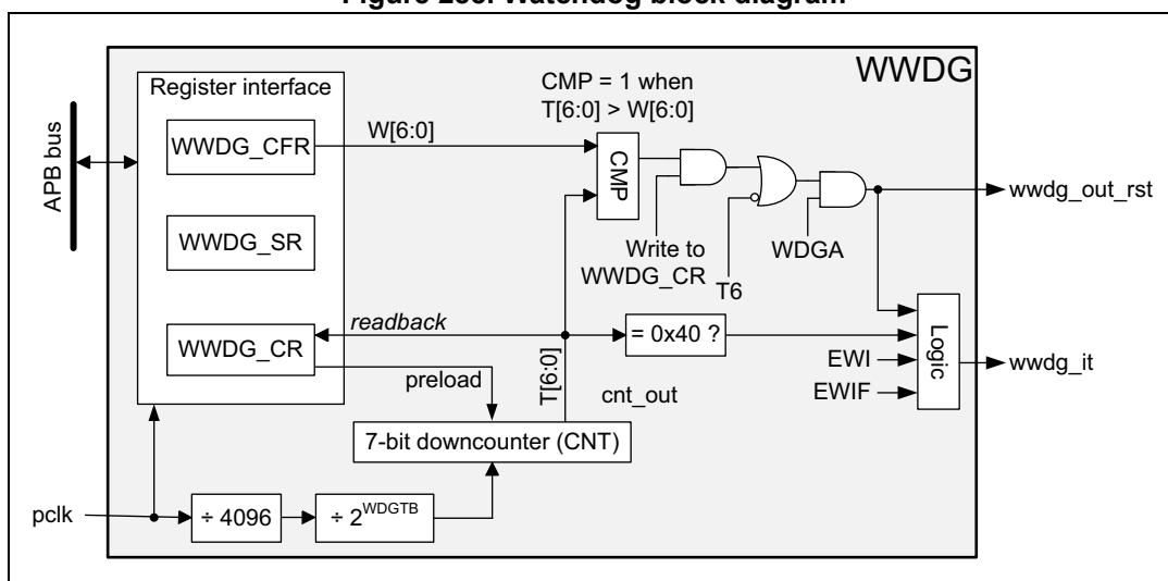
Figure 288. Watchdog block diagram
