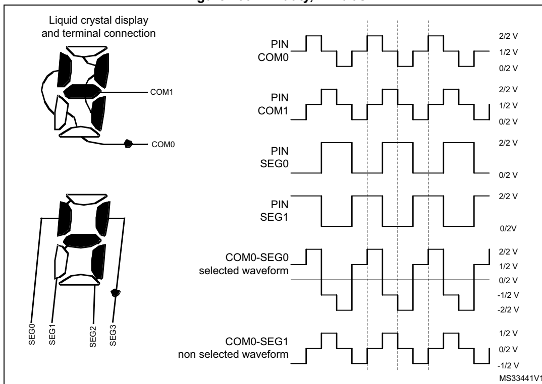
Figure 100. 1/2 duty, 1/2 bias
