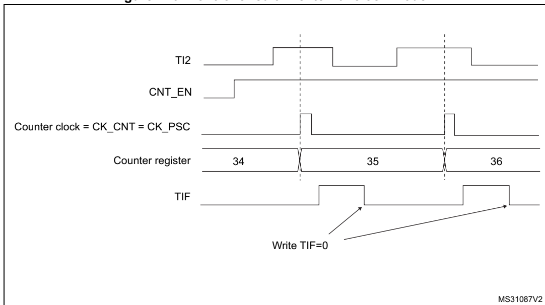
Figure 226. Control circuit in external clock mode 1
