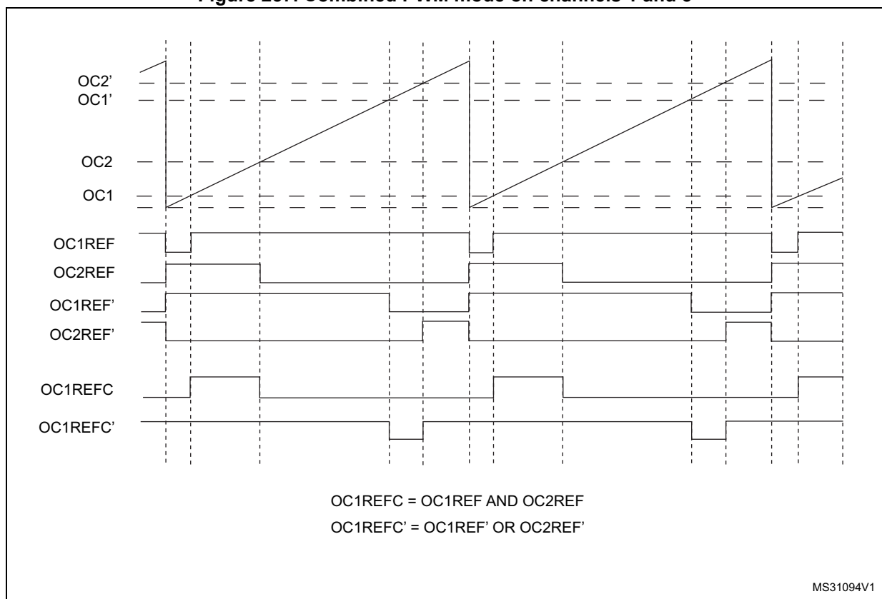
Figure 237. Combined PWM mode on channels 1 and 3
