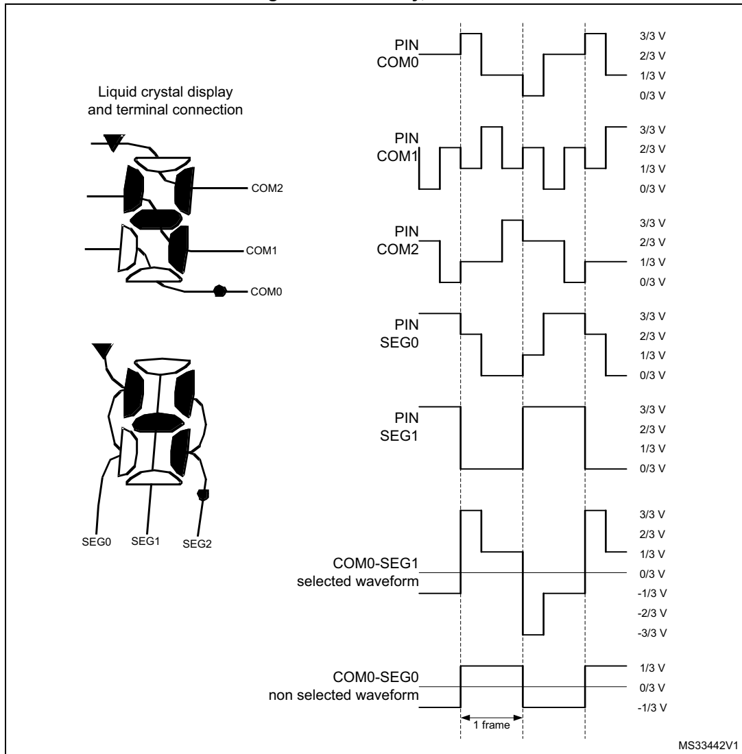
Figure 101. 1/3 duty, 1/3 bias
