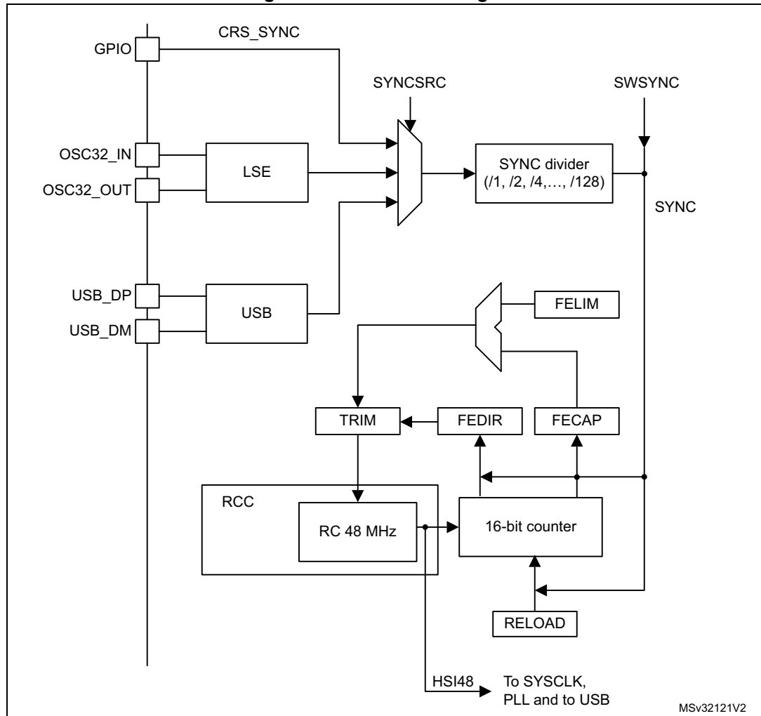
Figure 410. CRS block diagram
