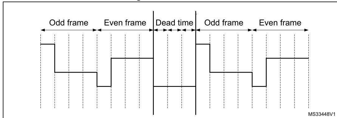
Figure 105. Deadtime
