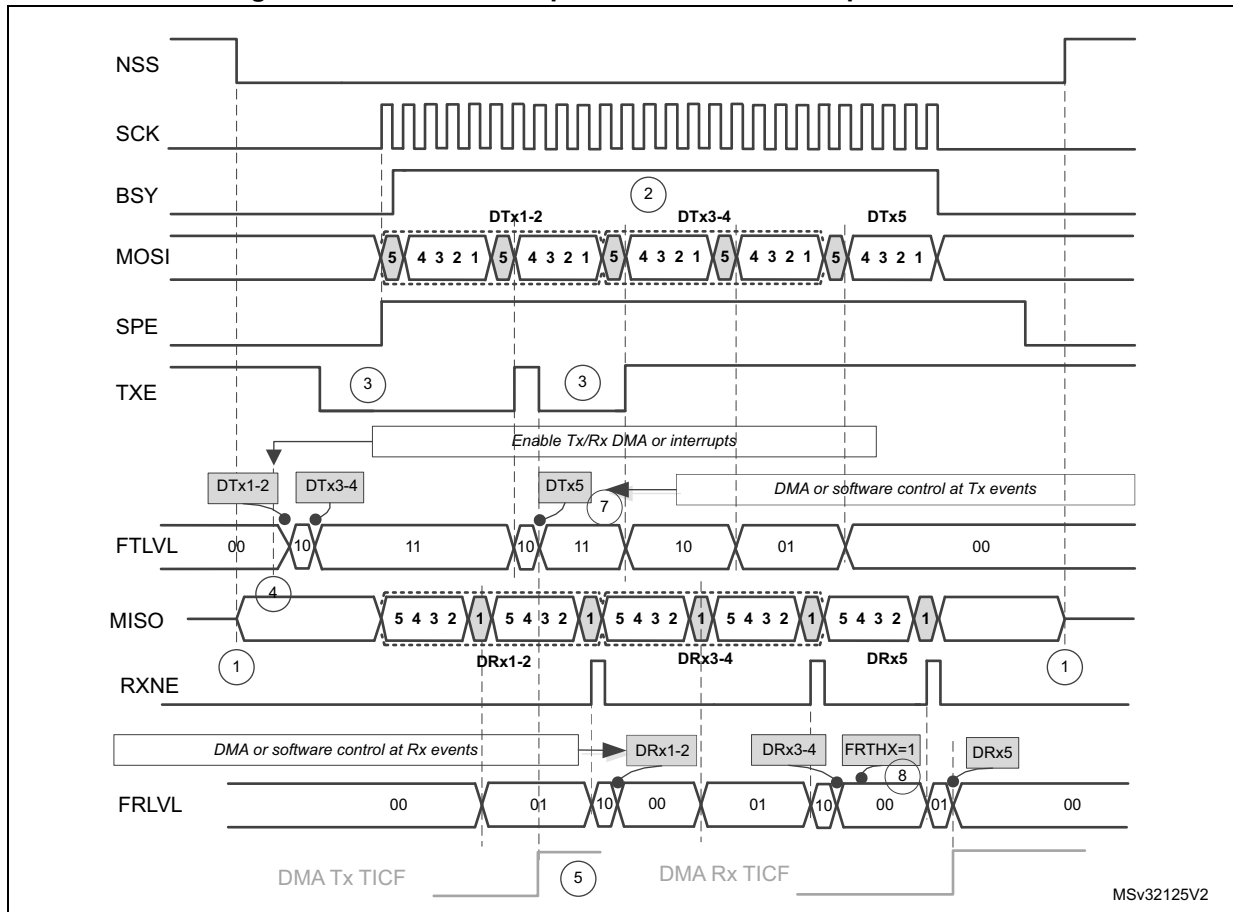
Figure 374. Master full-duplex communication in packed mode
