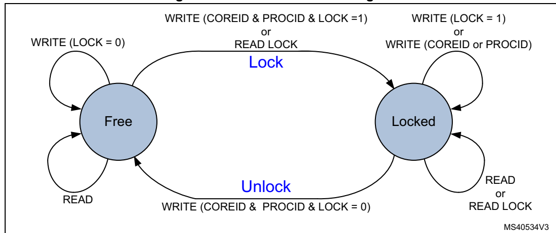
Figure 406. Procedure state diagram
