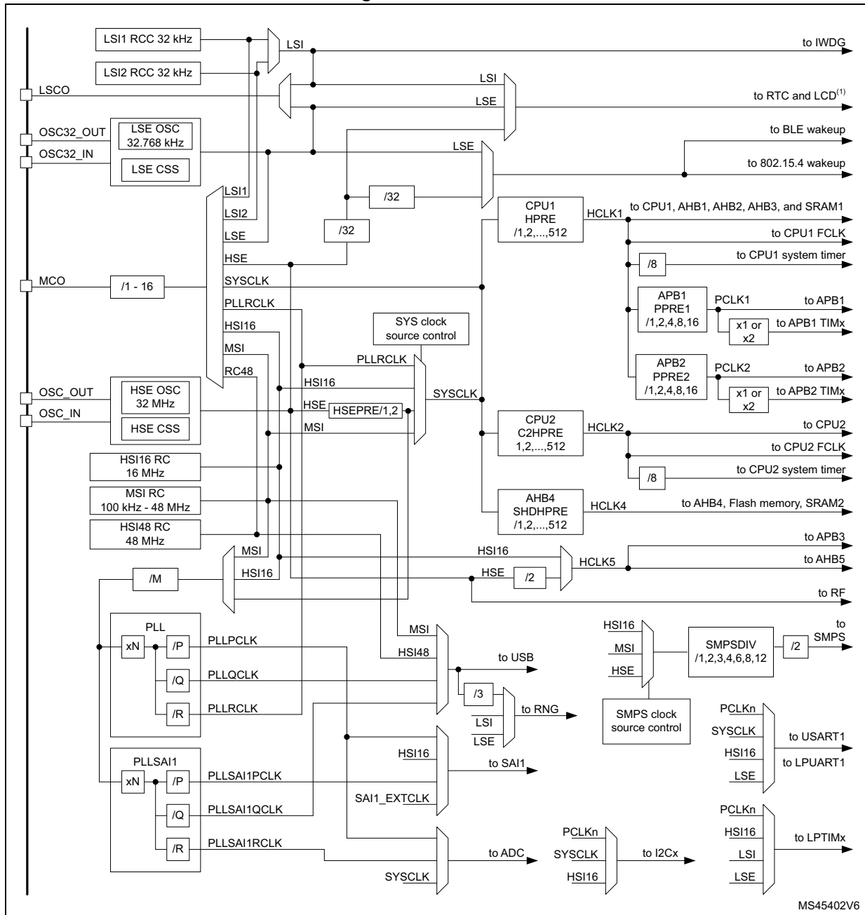
Figure 15. Clock tree
