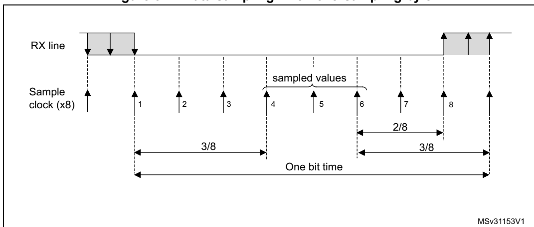
Figure 327. Data sampling when oversampling by 8
