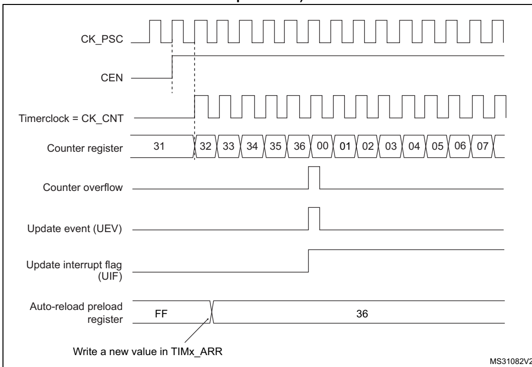
Figure 211. Counter timing diagram, Update event when ARPE=0 (TIMx_ARR not preloaded)
