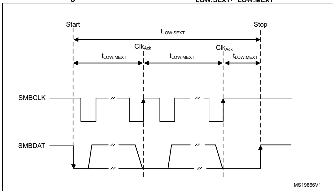
Figure 313. Timeout intervals for t_{LOW:SEXT} , t_{LOW:MEXT}
