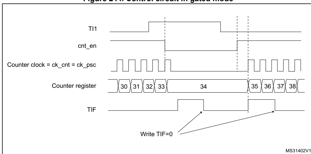
Figure 244. Control circuit in gated mode
