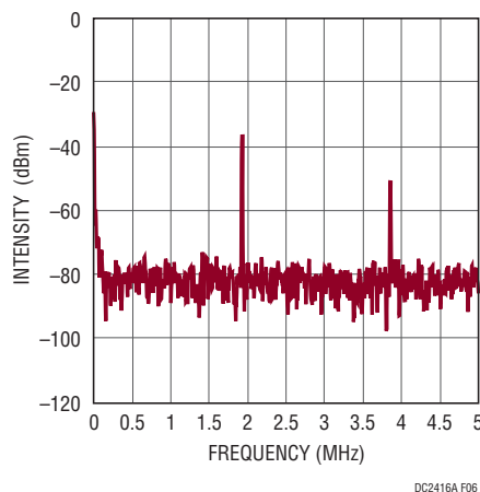
Figure 6. Output Noise Spectrum with 3.5A Load Current ( V_{IN} = 12V )
