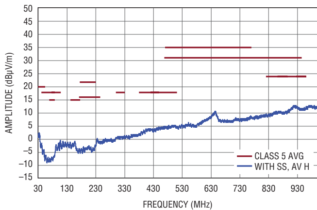
(3a) Horizontal Polarization, Average, with Spread Spectrum
