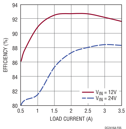
Figure 5. DC2416A Efficiency vs Load Current ( T_A = 25^\circ C )
