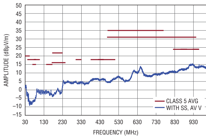
(3b) Vertical Polarization, Average, with Spread Spectrum
