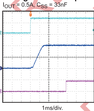
Power Good through EN Start Up
