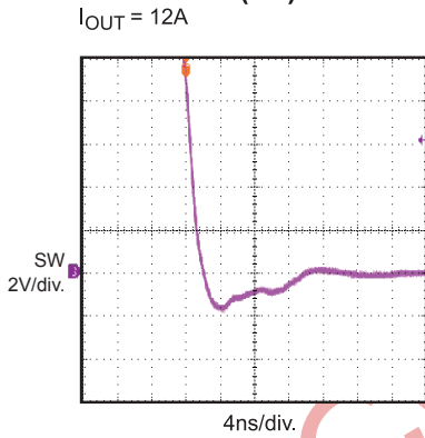
Dead Time (off)
