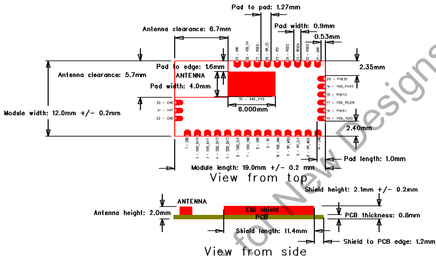
Figure 9.1. Physical Dimensions
