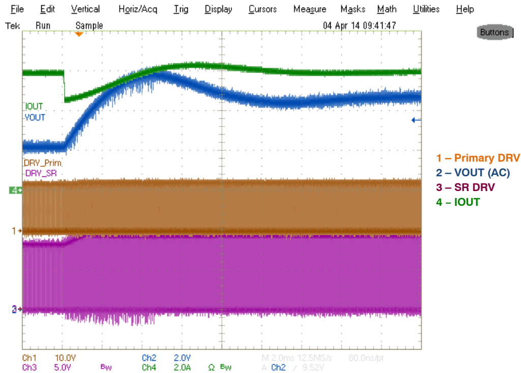
Figure 29. V_{IN} = 230 V_{AC} , I_{OUT} = 8.0-10.5 A
