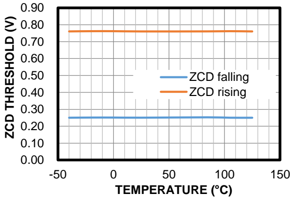
ZCD Threshold vs. Temperature
