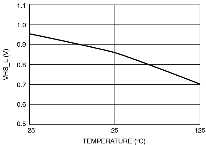
Figure 21. High-Side Drive Voltage vs. Temperature (low state, Isink = 100 mA, @ Vbst = 25 V)
