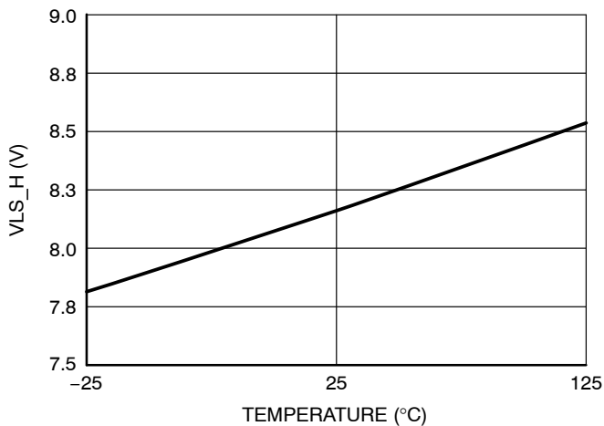
Figure 23. Low-Side Drive Voltage vs. Temperature (high state, Isource = -500 mA, @ VDD = 10 V)
