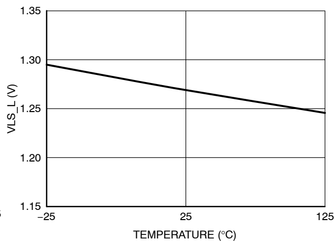
Figure 24. Low-Side Drive Voltage vs. Temperature (low state, Isink = 750 mA, @ VDD = 10 V)
