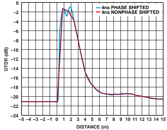
Figure 97. Comparison of Closely Spaced Event Detection with and Without Phase Shifting, 4 ns Pulse Width, 1 m Event Separation
