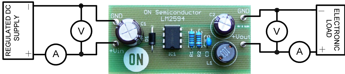
Figure 1: Test Setup
