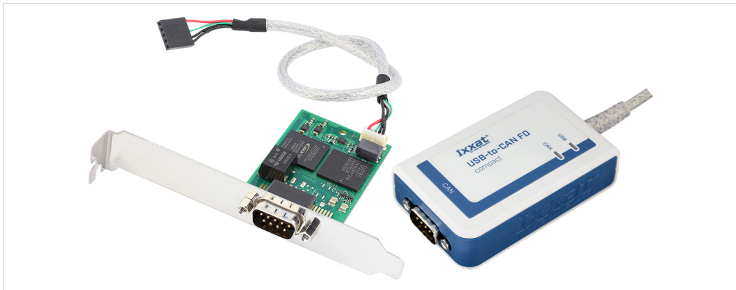
Fig. 1 USB-to-CAN FD embedded and compact (D-Sub 9)
