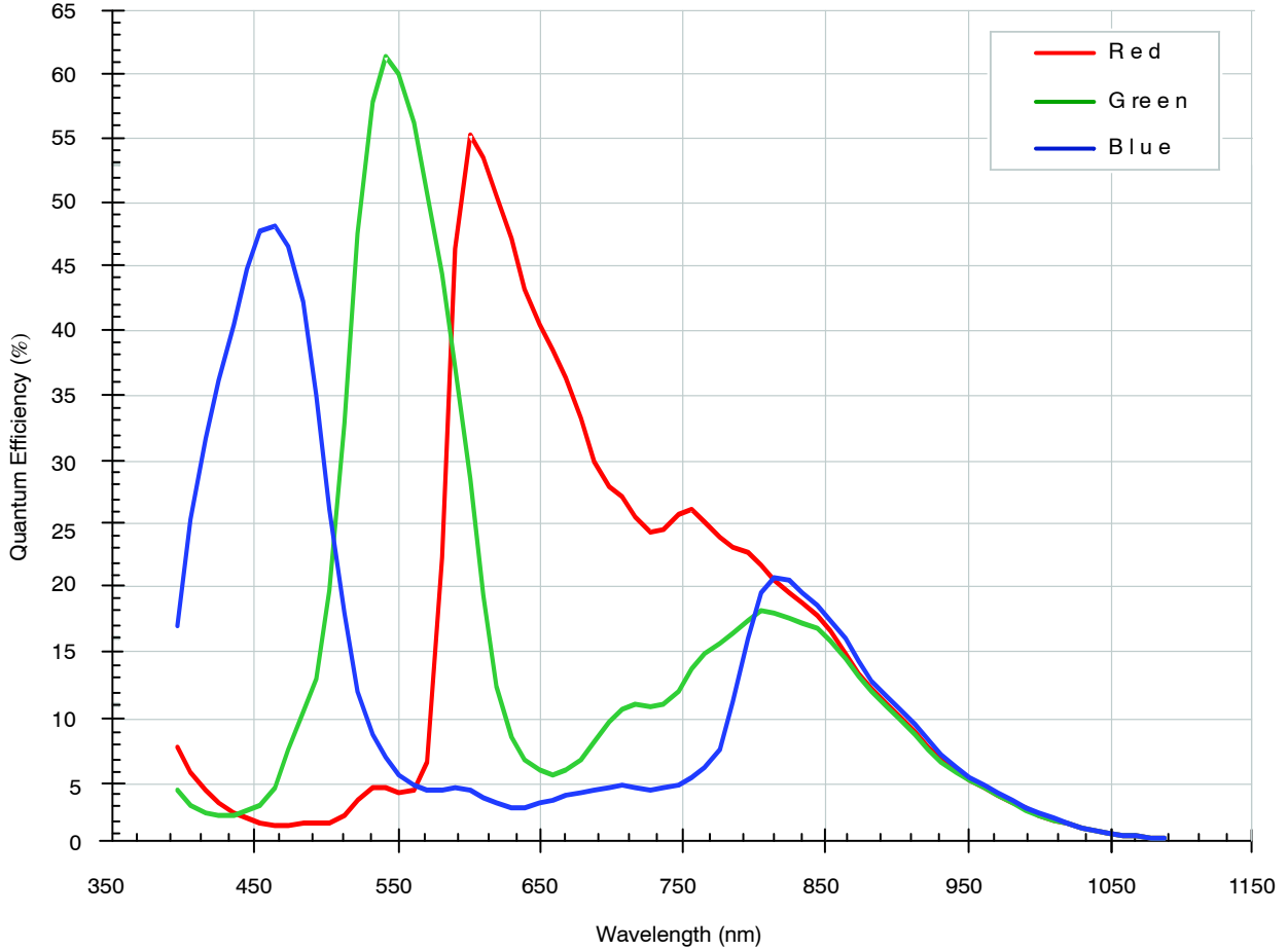
Figure 43. Quantum Efficiency
