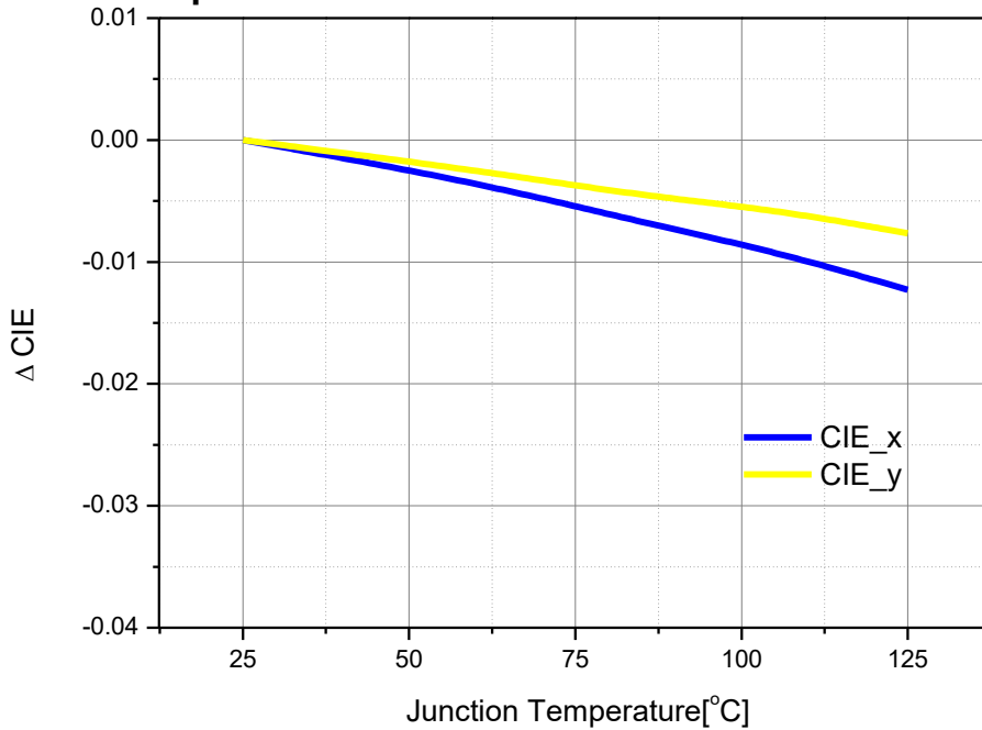
Junction Temperature vs. White \Delta CIE at IF=700mA
