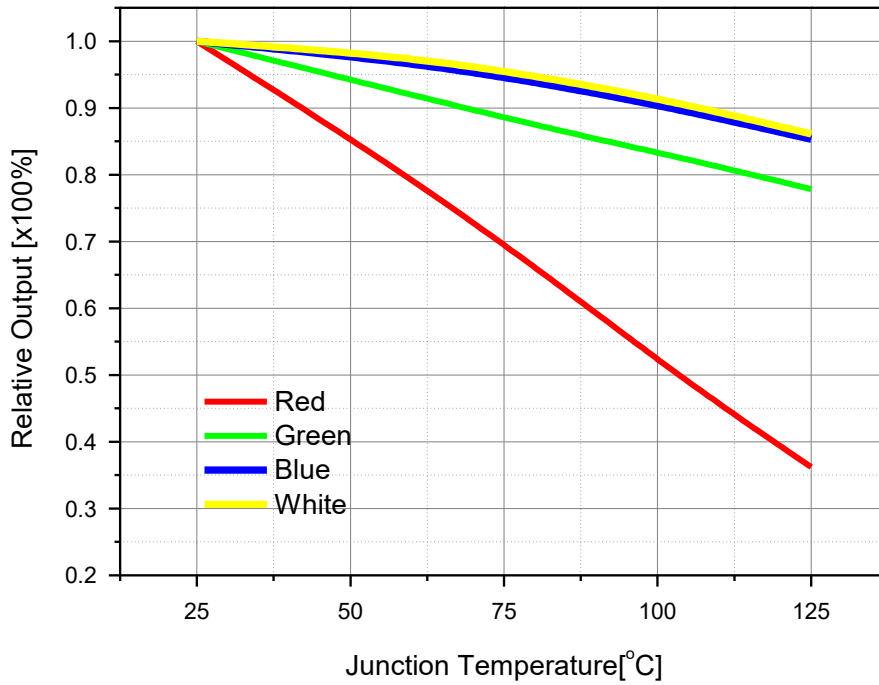
Junction Temperature vs. Relative Light Output at IF=700mA
