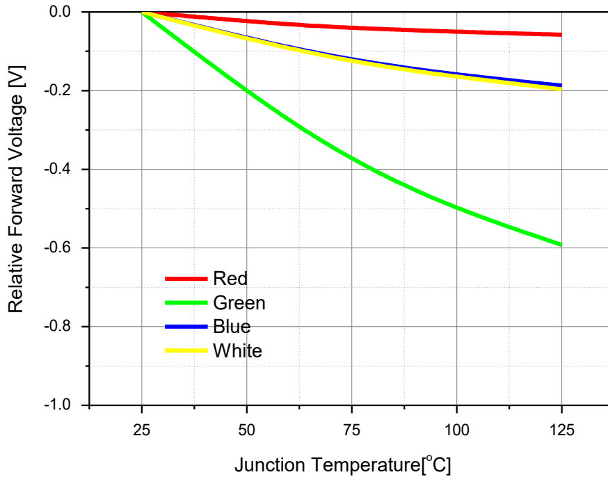
Junction Temperature vs. Forward Voltage at IF=700mA
