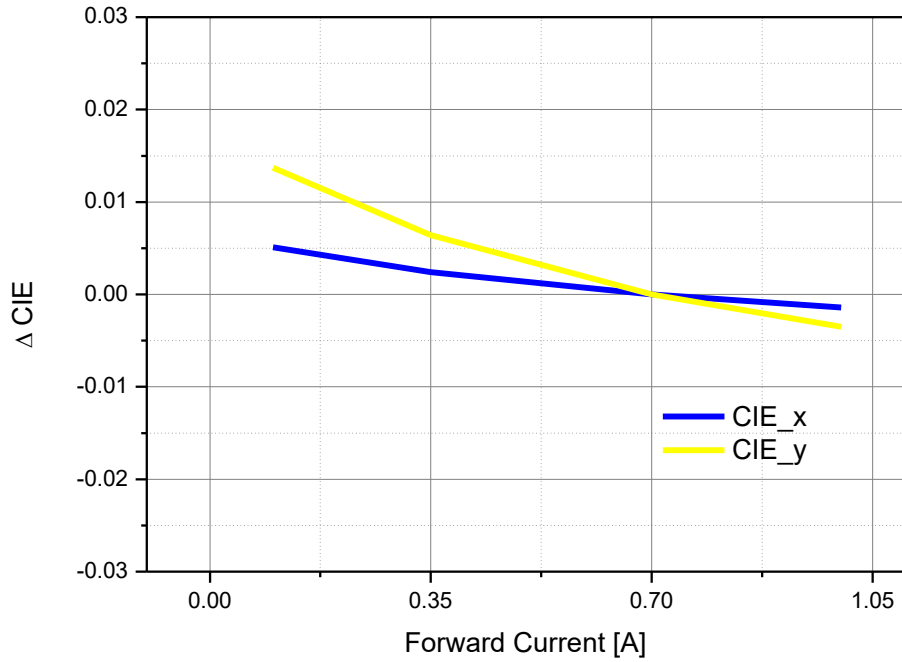
Forward Current vs \Delta CIE, T_j=25^\circ\text{C} (White)
