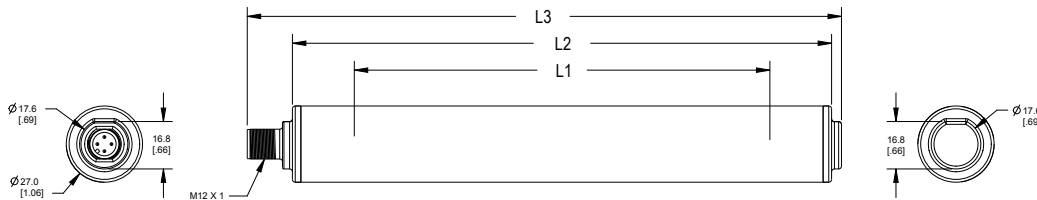
Figure 4. Cascade Models
