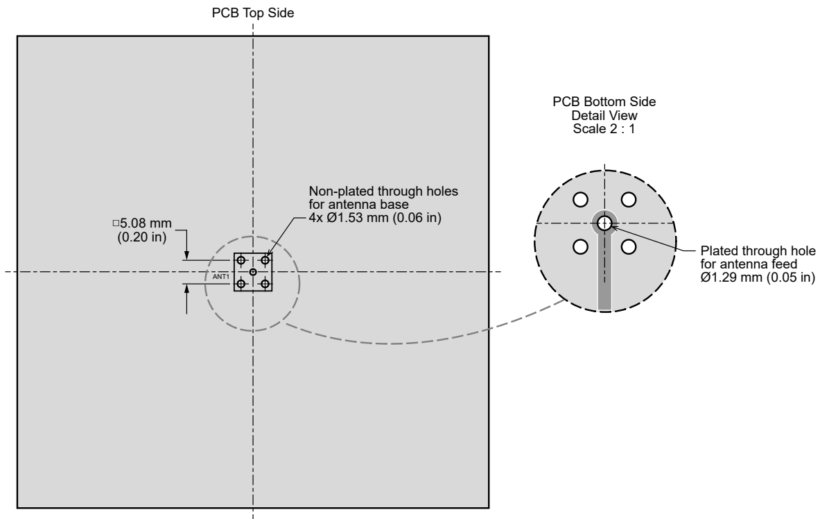
Figure 10. ANT-868-VHETH Antenna Placement on PCB
