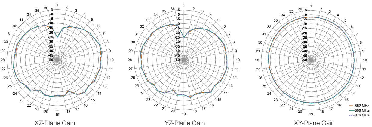
Figure 7. ANT-868-VHETH Antenna Radiation Patterns
