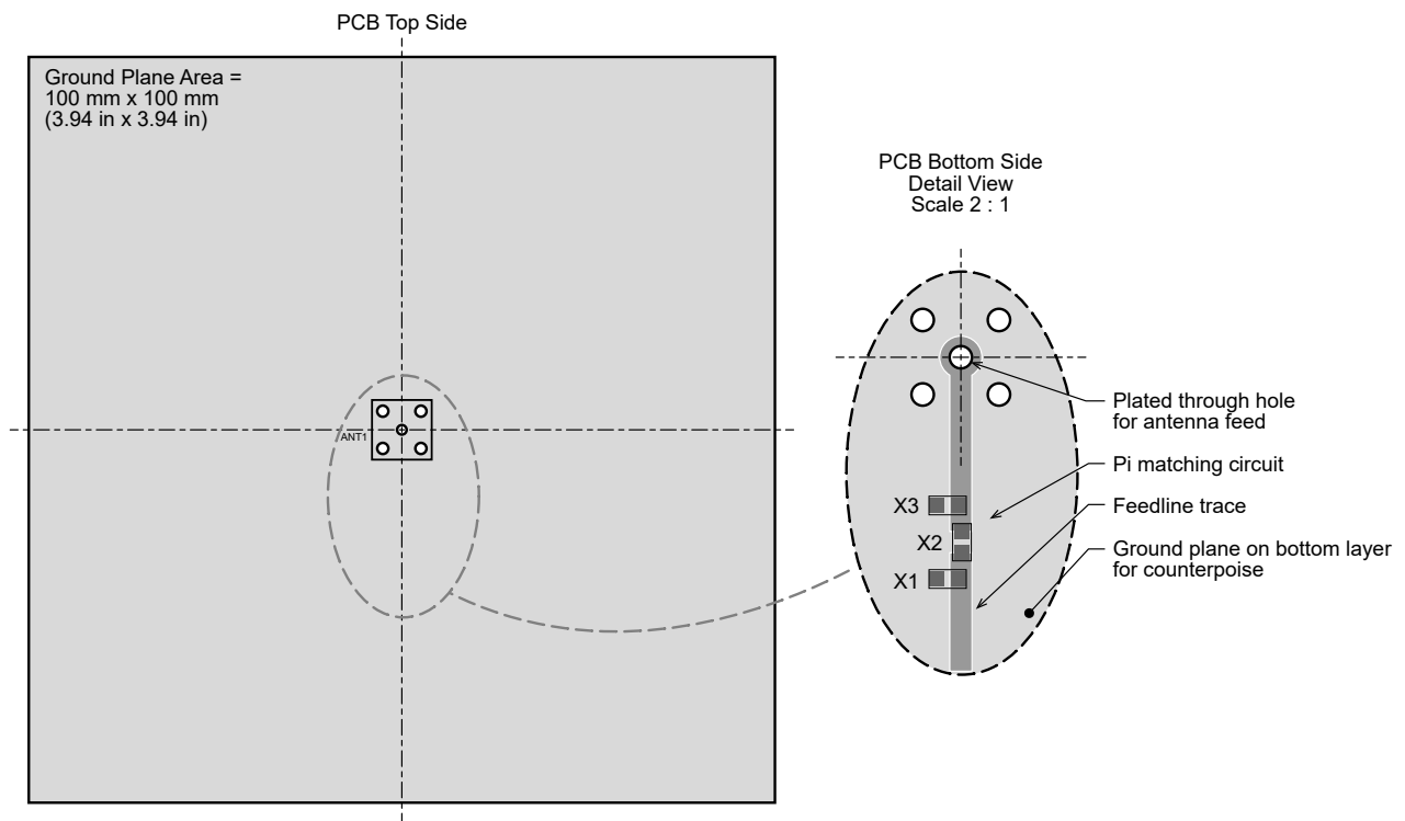
Figure 8. ANT-868-VHETH Recommended Layout
