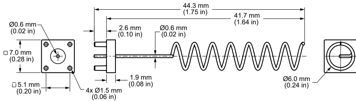
Figure 1. ANT-868-VHETH Antenna Dimensions
