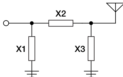
Figure 9. Matching Network Recommendation
