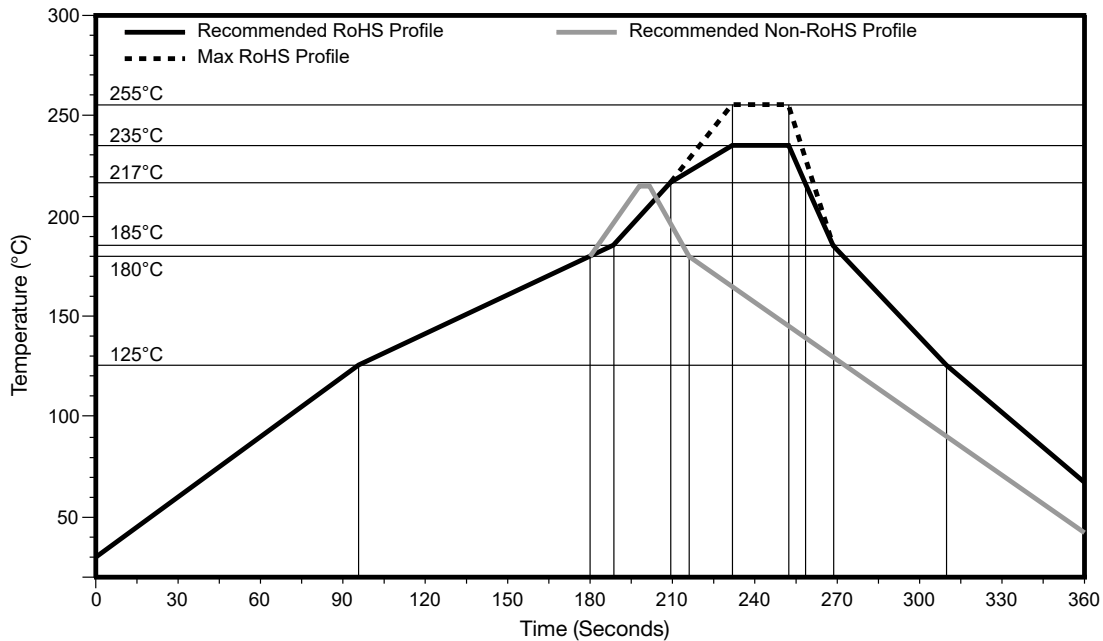
Figure 11. Solder Profile for the ANT-868-VHETH Antenna
