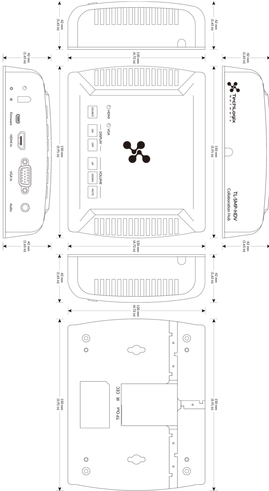
Receiver Dimensional Drawing
