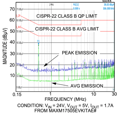
CONDUCTED EMISSION PLOT WITH FILTER: C4 = 2.2µF, L1 = 10µH, C14 = 2.2µF
