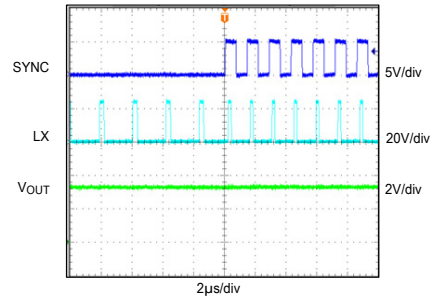
SYNC FREQUENCY AT 740 KHZ V_{IN} = 24V, V_{OUT} = 5V, I_{OUT} = 0A, MODE = GND
