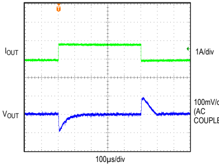
LOAD CURRENT TRANSIENT RESPONSE V_{IN} = 24V, V_{OUT} = 5V, I_{OUT} = 0.05A - 0.85A, MODE = VCC
