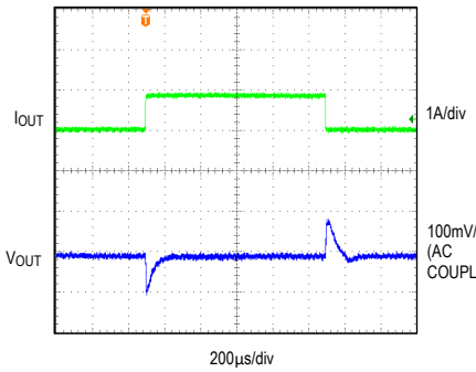
LOAD CURRENT TRANSIENT RESPONSE V_{IN} = 24V, V_{OUT} = 3.3V, I_{OUT} = 0.05A - 0.85A, MODE = VCC
