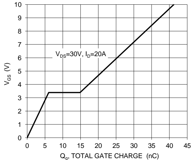
Figure 10. Gate Charge
