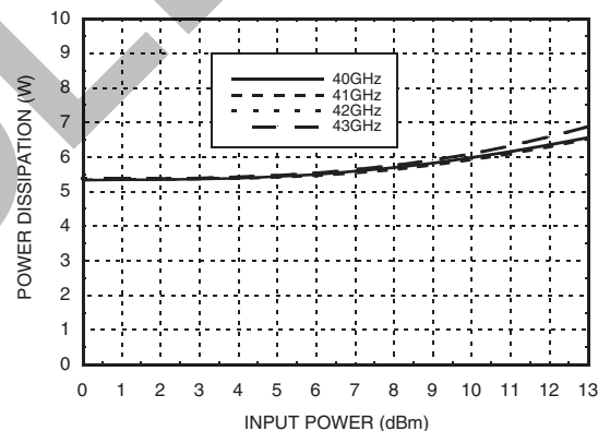
Power Dissipation
